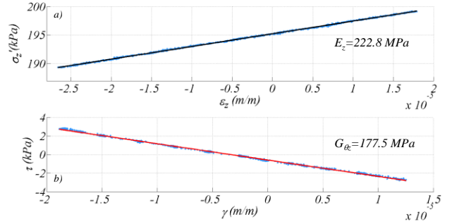
Fig. 8 Stress and strain relationship for a single cycle of q=\pm 5 kPa: in axial direction (a) with relative Elastic ( E_z ) modulus and in torsional direction (b) with Shear moduli ( G_{\theta z} ) measured at the ip of test 2.
