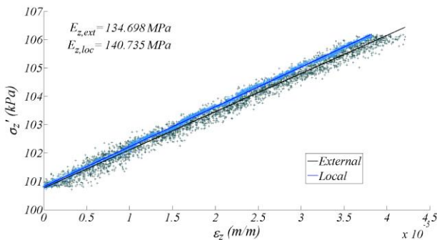
Fig. 7 Young modulus ( E_z ) measured in triaxial compression and extension: comparison local and external strain measurement systems.
