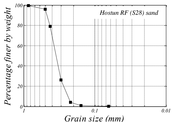
Fig. 1 Grain size distribution, Hostun RF (S28) sand [2].
