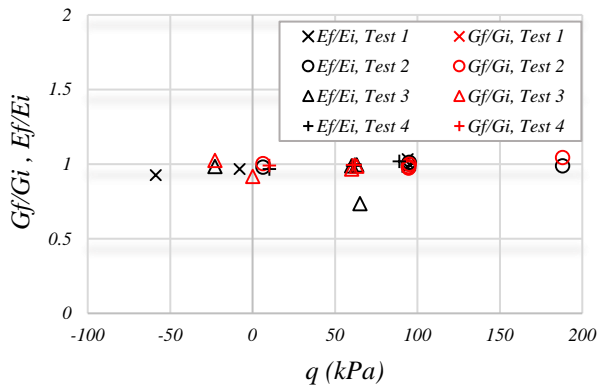
Fig. 10 Elastic ( E_z ) and Shear moduli ( G_{\theta z} ) ratio between initial and final investigation points (ip) for each test.
