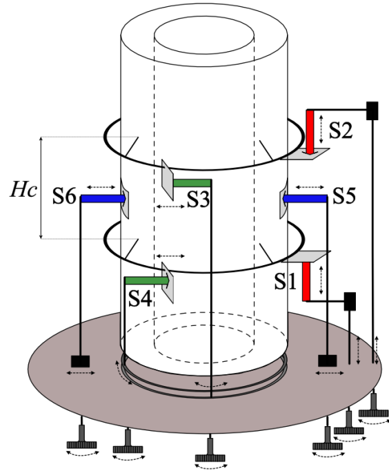
Fig. 3 Schematic view on the small strain measurement system around the hollow cylindrical specimen.
