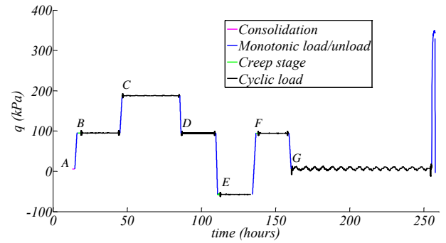
Fig. 5 Evolution of the deviatoric stress ( q ) for the performed experimental programme.
