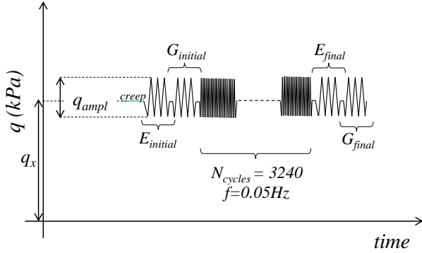
Fig. 6 Schematic representation of cyclic loading procedure applied.
