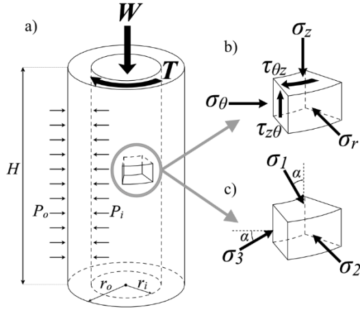
Fig. 2 Stress state in hollow cylinder torsional sample (a). Details of the element in the wall: (b) the stress components and (c) main principal stresses.
