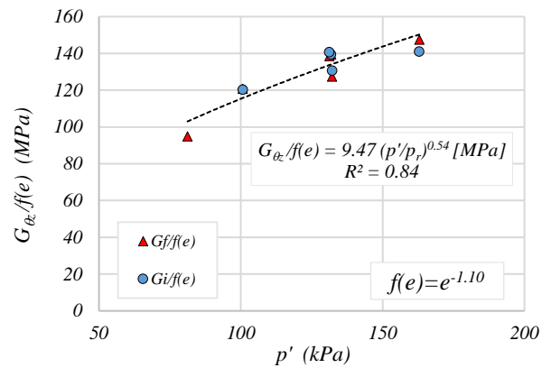
Fig. 9 Shear moduli ( G_{\theta z} ) compare with mean pressure for test 2 ( p_r represents a reference pressure of 1 kPa).
