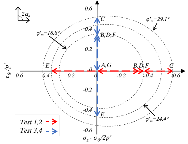
Fig. 4 Imposed stress path in the normalized shear stress-deviatoric stress plane.
