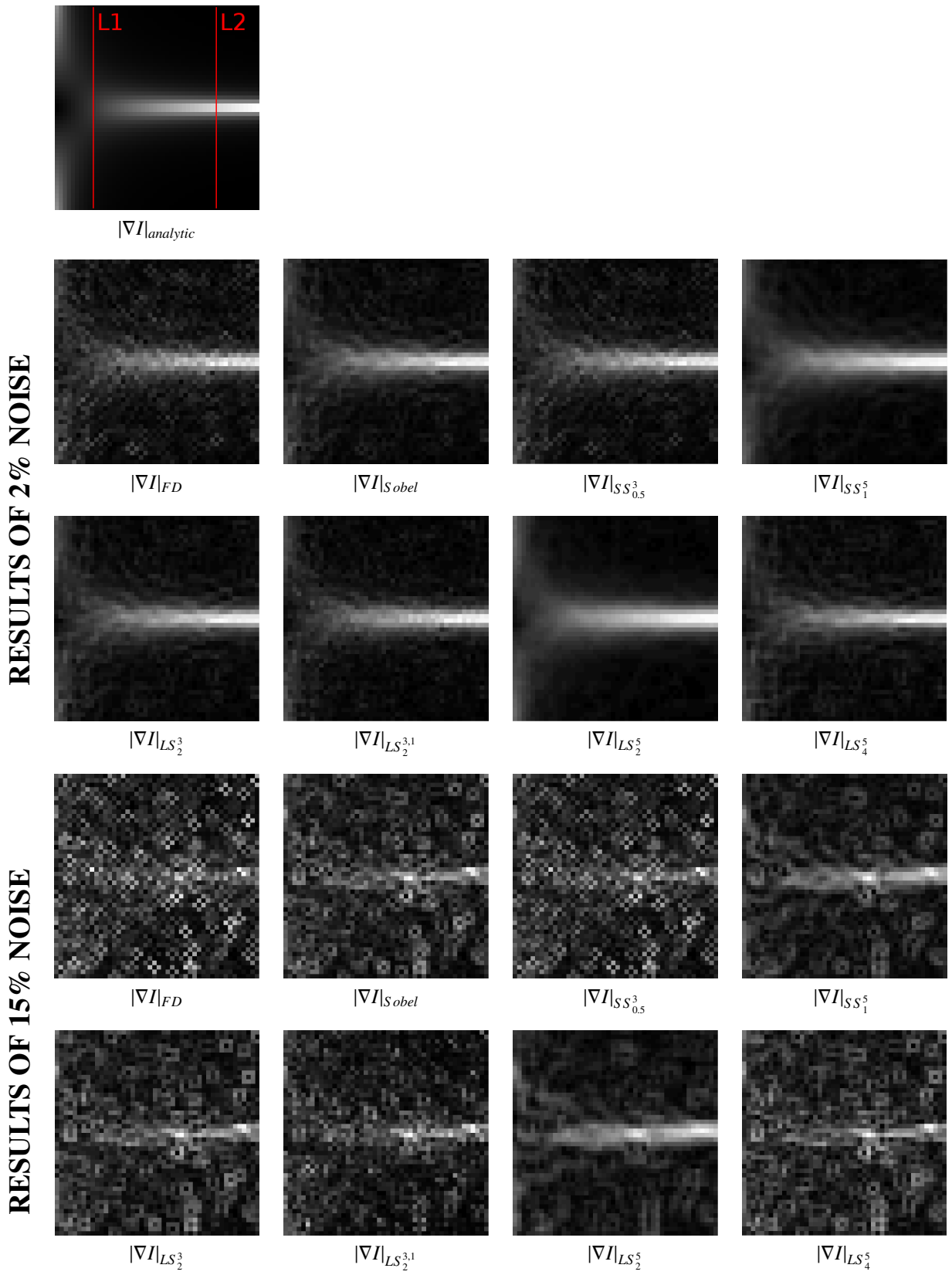
Figure 3: Gradient magnitude of the arctan image , computed using different approaches as discussed in section 3. Top row: analytic solution of the image gradient magnitude; rows 2-3: results for image with 2% noise; rows 4-5: results for image with 15% noise.
