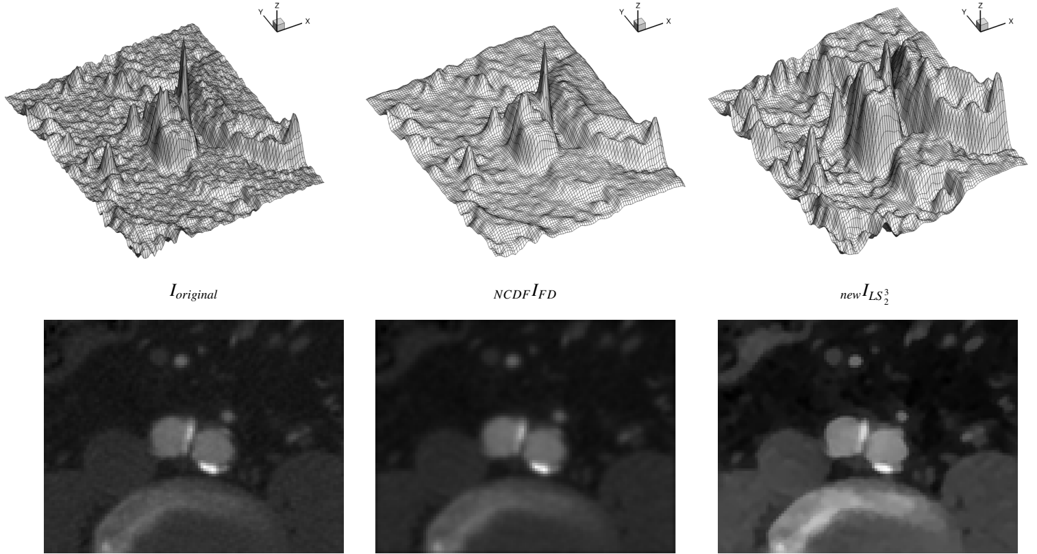
Figure 12: Results of the image processing on the abdominal CTA image test. Top row show the visualisation of the image as a topographic landscape.
