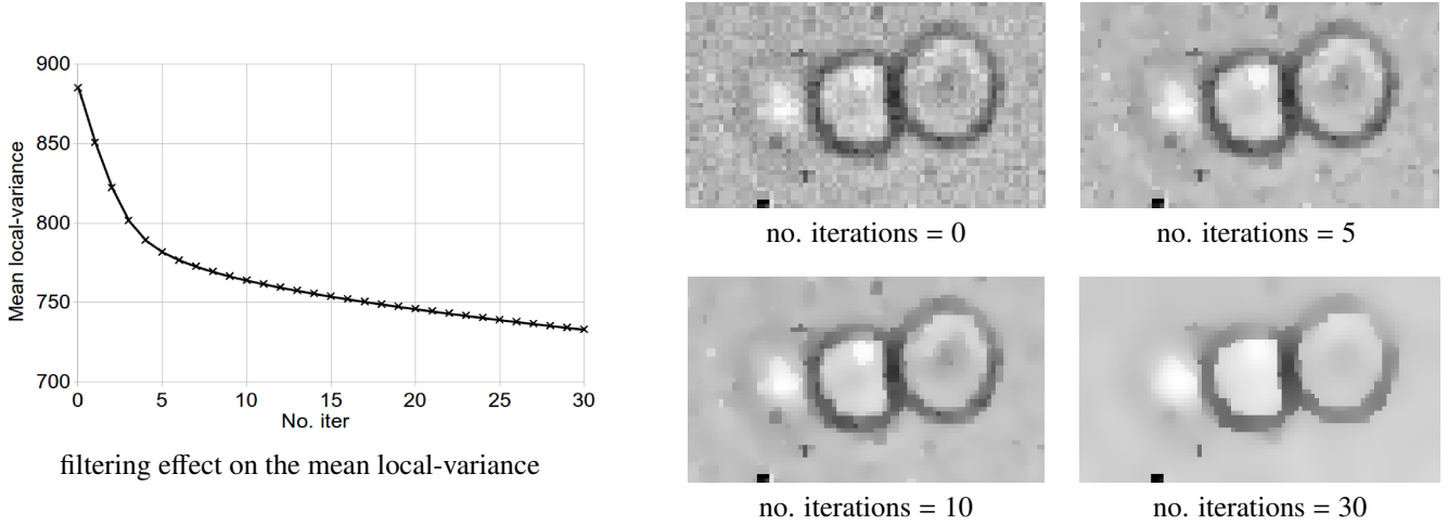
Figure 5: Results of filtering the microscopy image test case using the PM method (equation 12). The mean local-variance is seen to decrease rapidly until approximately 5 iterations, and then continue decreasing at a different rate. The optimal filtering is at the end of the initial stage, hence around 5 iterations. Here \beta = 10 and the integration time step is dt = 1/7 .
