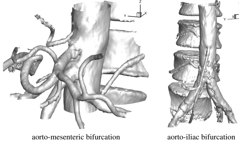
Figure 7: Extracting the zero-level iso-surface of the inflection point criterion (3D extension to equation 18) for the descending aorta CTA dataset (unprocessed). Note that aorta and iliac arteries have nodular irregularities, that correspond to atherosclerotic plaque. For clearer visibility, surrounding structures as well as features with |\nabla I| < 3 (units: normalised intensity per unit pixel) are removed (in an automated process with minimal user intervention).
