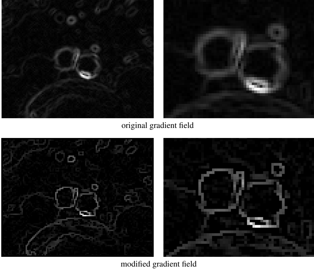
Figure 6: Gradient magnitude of the abdominal CTA image . Top row: original; bottom row: modified using equation 14. Right column shows detail of the image. The processing on the gradient field can be seen to be drastic. The reconstructed image is shown in figure 12.
