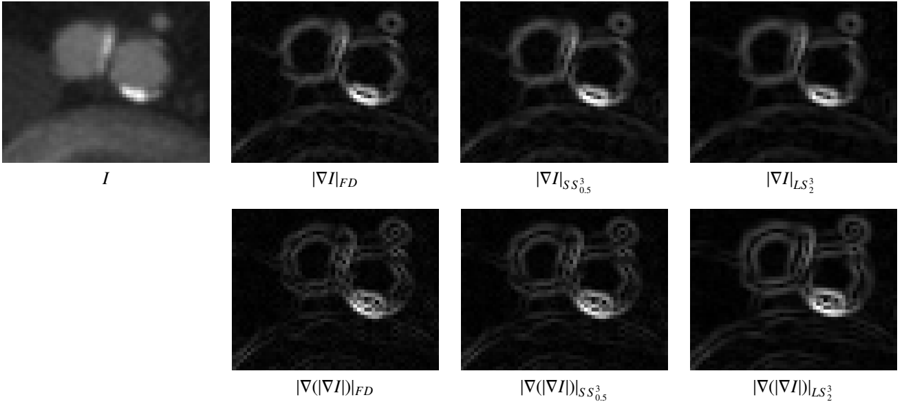
Figure 4: Comparison of the effectiveness of calculating spatial derivatives, using the abdominal CTA image test case. Results for |\nabla(|\nabla I|)| are obtained by initially computing |\nabla I| . LS^3_2 method proves to have smoother results.
