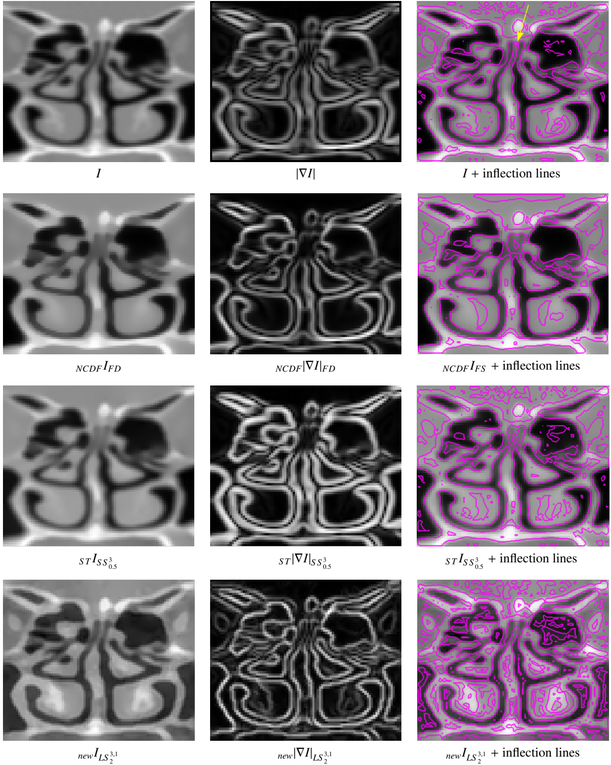
Figure 13: Results of the image processing on the cranial CT image test. Lines of inflection are shown (equation 18), which were computed from the images using the LS_2^3 approach on the output image.
