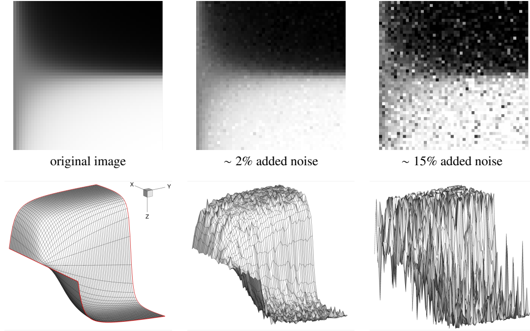
Figure 2: Synthetic image of the arctangent function (equation 1-2), without noise and with noise ( \sim 2\% and \sim 15\% of the signal amplitude). Top row: scaled image; bottom row: visualisation as topographic landscape.
