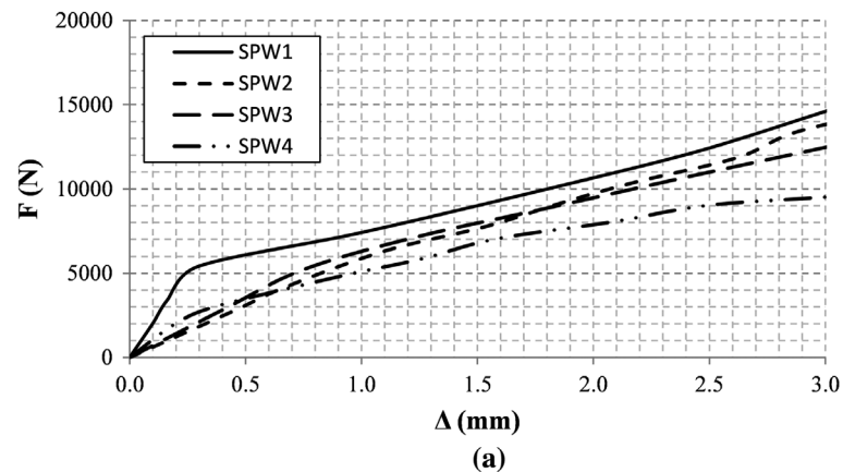
Figure 7. Experimental initial curves of the panels tested by Valizadeh et al. (2012) having thickness equal to 0.70 mm (a) and (b) 0.37 mm (b). Despite a larger hole diameter, SPW8 panel showed an apparently initial curve stiffer than the other perforated panels: this may be due to the initial slipping under the first load increment.
