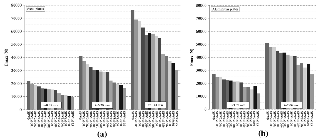
Figure 9. Comparison between analysed steel panels (a) and aluminium panels (b) in terms of shear strength.
