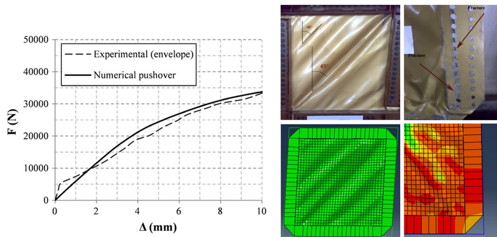
Figure 6. Experimental-numerical comparison of force-displacement curves and numerical calibration in terms of deformed shape and stress concentration related to the SPW1 specimen tested by Valizadeh et al. (2012).
