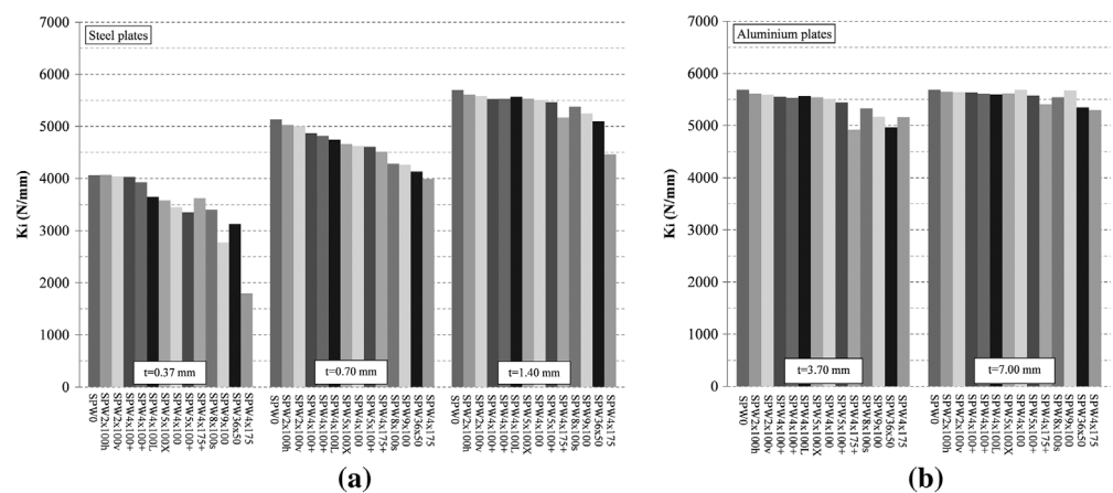
Figure 10. Comparison between analysed steel panels (a) and aluminium panels (b) in terms of initial stiffness.
