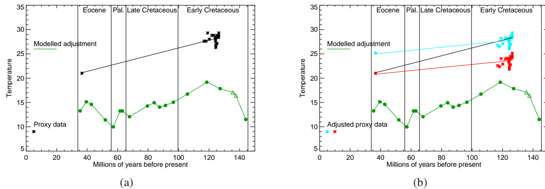
Figure 10. (a) Proxy temperature data (black asterisks) at Falkland plateau (Site 511) from \text{TEX}_{86} . Eocene data are from Liu et al. (2009), and Cretaceous data from Jenkyns et al. (2012). Black line shows the line of best fit. Also shown is the modelled temperature evolution at Falkland plateau (green line), i.e. the adjustment factor. In (b), the proxy data have been adjusted using the model output, relative to either the earliest (light blue) or latest (red) proxy data point. Blue and red lines show the respective lines of best fit. \text{TEX}_{86} temperatures are calculated using the \text{TEX}_{86}^H -SST calibration of Kim et al. (2010).
