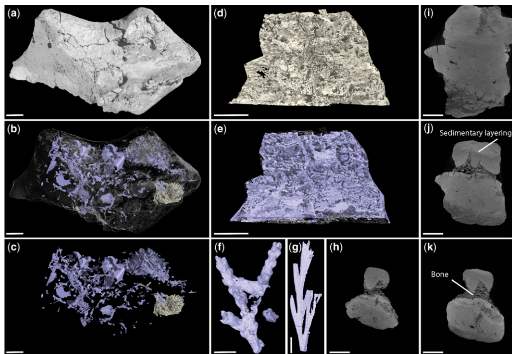
Fig. 5. Computed tomography reconstructions of: (a) the endocranium (lateral view from the right side); (b, c) voids/regions of lower density within the endocranium; (d) a bone fragment at the back of the endocranium (dorsal view); (e) the voids within the bone fragment (interpreted as Haversian canals or trabeculae); (f) a branching twig within the sediment infill; and (g) a leaf within the sediment infill. (h–k) Representative computed tomography slices through the endocranium revealing regions of bone and layering within the sediment infill. All reconstructions in this figure were generated using the SPIERS software suite and were rendered in Blender. Scale bars: (a–c, h–k) = 10 mm, (d, e) = 5 mm, (f, g) = 2 mm.
