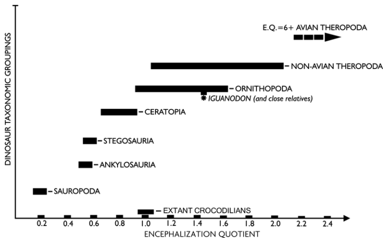
Fig. 10. Encephalization quotients (EQ) estimated across a range of dinosaur clades/groupings. Extant crocodylians represent the reference marker (EQ = 1.0) for comparison with dinosaurians more generally. Ornithopods (such as Iguanodon and closely related taxa) exceed the EQ of extant crocodylians and overlap the values seen in basal (non-avian) theropods. Modified from Hopson (1979).
