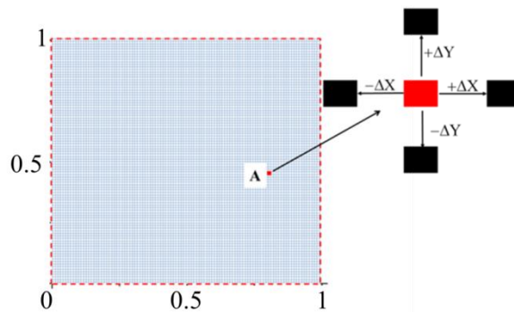
Fig. 4. Schematic of the discretization process used to calculate GND density. The plastic deformation gradient ( \text{curl } F^p ) is calculated in each discretized region using the detailed non-local approach similar to that adopted by [1].
