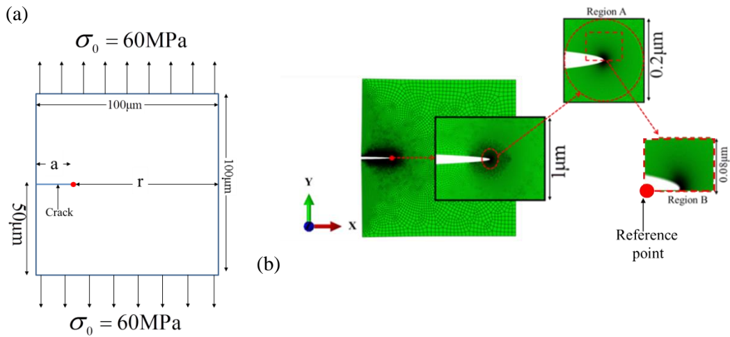
Fig. 2. (a) Schematic of 100 \times 100 \mu\text{m}^2 2-D single crystal plate with an embedded edge crack of length a = 20 \mu\text{m} . The plate is meshed as shown in (b) and two regions of interest are defined. Region A is circular with diameter 0.2 \mu\text{m} and Region B is a subset of A and has dimensions 0.08 \times 0.08 \mu\text{m}^2 .
