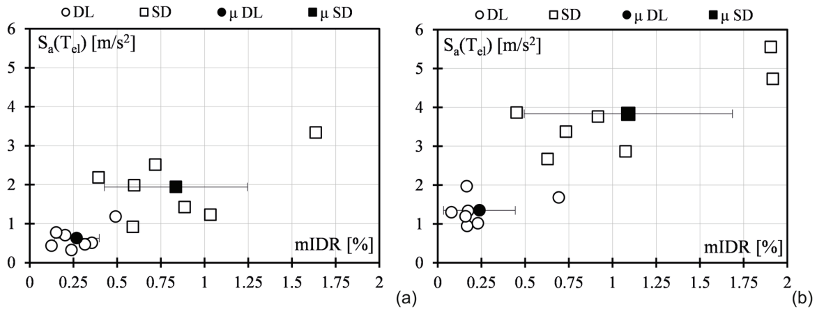
Figure 9. IM-EDP results in X direction (a), and Y direction (b) (Adapted from De Luca et al., 2014)
