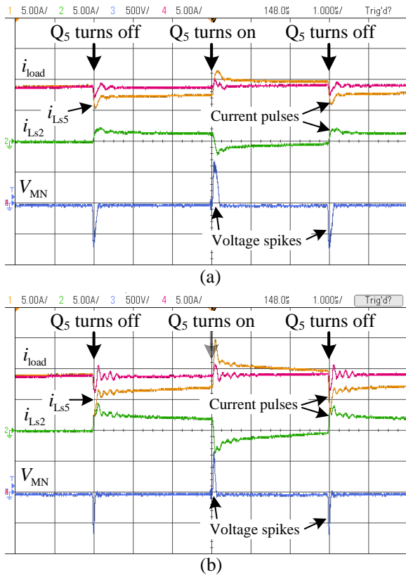
Fig. 13. Current pulses and voltage spikes of the split inductors with split inductance of (a) 10µH and (b) 2.5µH.
