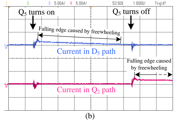
Fig. 12. The charging, discharging, and freewheeling currents: (a) without split inductors and (b) with split inductors of 10\mu\text{H} .
