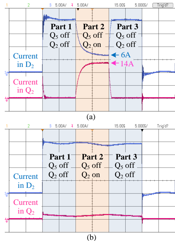
Fig. 14. Synchronous rectification: (a) without split inductors and (b) with split inductors of 10µH.
