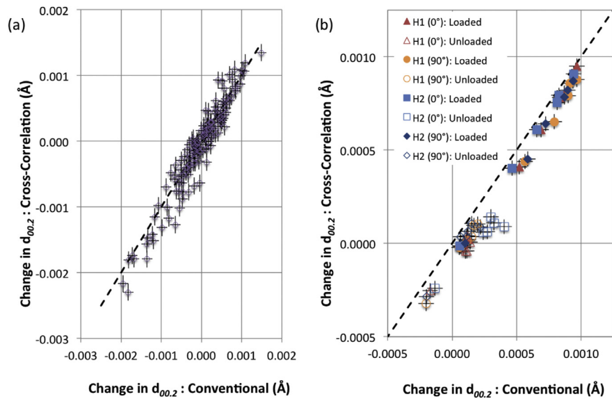
Fig. A4. Comparison of the shift in d_{002} measured by the conventional and cross-correlation methods for a) neutron diffraction, and b) synchrotron X-ray diffraction. The error bars are the expected uncertainty in the analysis, obtained for the signal to noise ratio of the d_{002} peak (Fig. A2).
