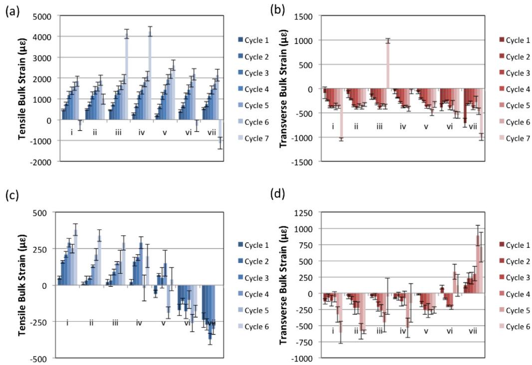
Fig. 5. The variation of axial and transverse strains across the gauge area, measured by image correlation of radiographs (module 3) for the 90° rotation at location H1 in the tensile specimen. The strains under load are presented in (a) for axial tensile strain and (b) transverse strain. The corresponding strains after unloading are presented in (c) and (d). The measurement locations, (i) to (vii) are indicated in Fig. 3b (bottom right). The error bars are obtained from the image correlation measurement uncertainty (one standard deviation). Note the differences in scale of the vertical strain axes. (A colour version of this figure can be viewed online.)
