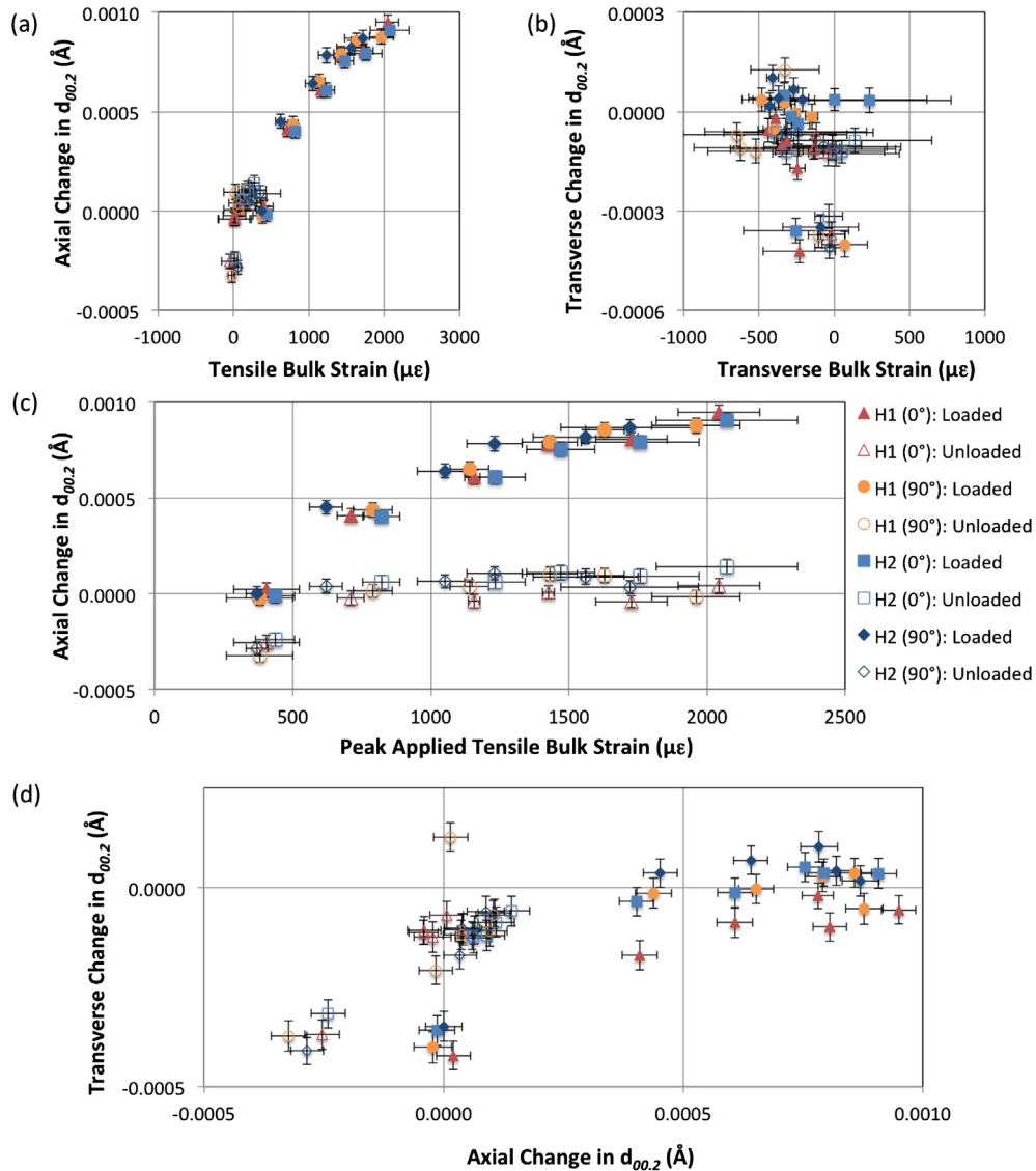
Fig. 10. The change in d_{(00.2)} : a) with the applied tensile bulk strain, b) at the transverse bulk strain both measured concurrently, c) as a function of the peak tensile bulk strain applied at or before the measurement; d) a comparison of the concurrent axial and transverse measurements. (Data shown for the loaded and unloaded state at locations H1 & H2, in the 0^\circ and 90^\circ orientations – see common legend). (A colour version of this figure can be viewed online.)
