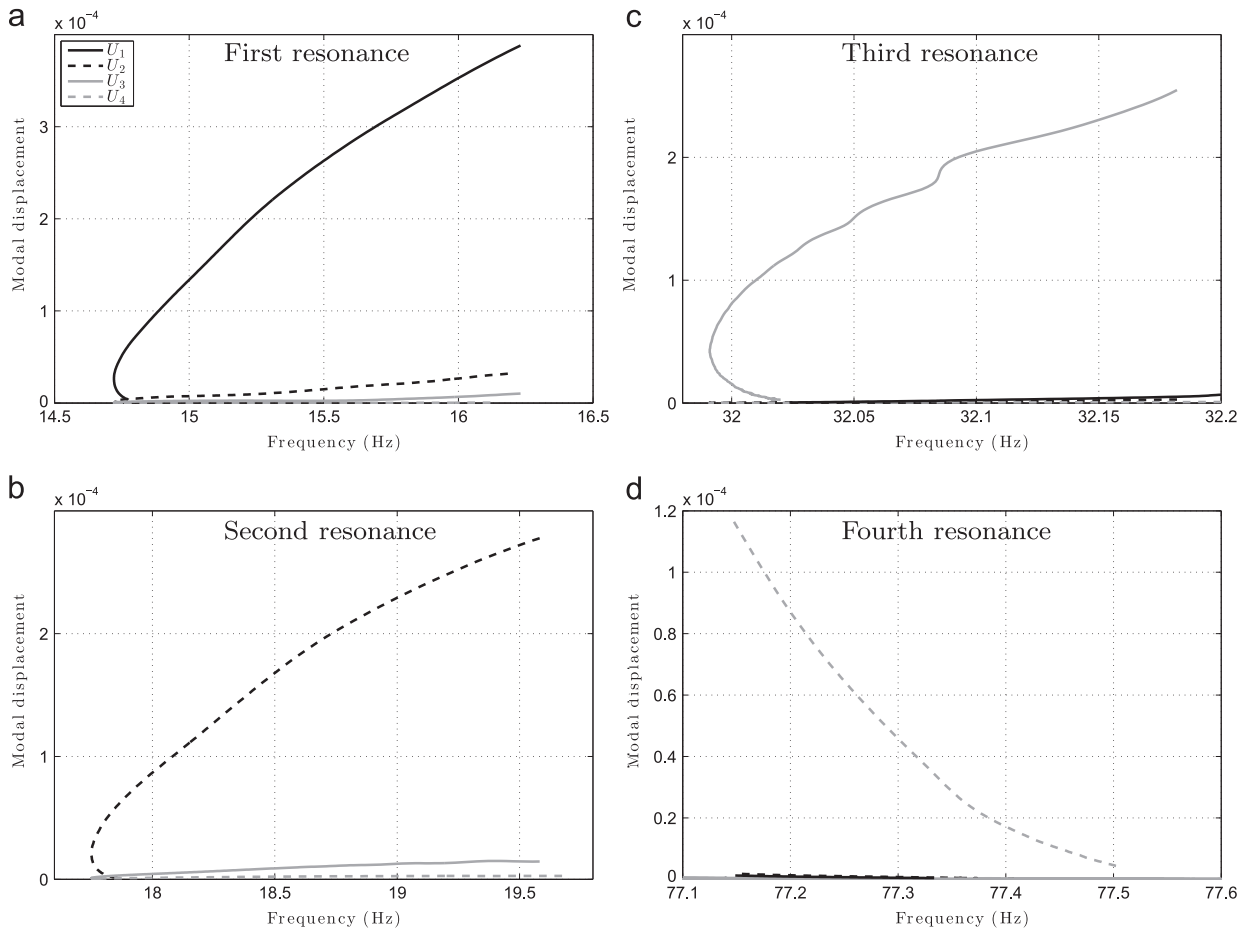
Fig. 13. Backbone curves estimated from experimental data in terms of the modal coordinates U_1 to U_4 .
