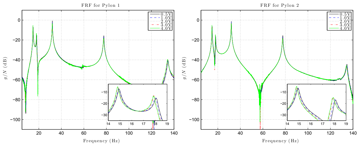
Fig. 11. Set of FRFs for either pylon ends at different levels of vibration using random excitation. Note the softening effect exhibited by the resonance peaks in the zoomed boxes.
