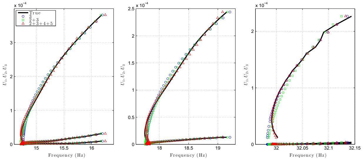
Fig. 14. Best fitting case of the trial models on top of the experimental backbone curves.
