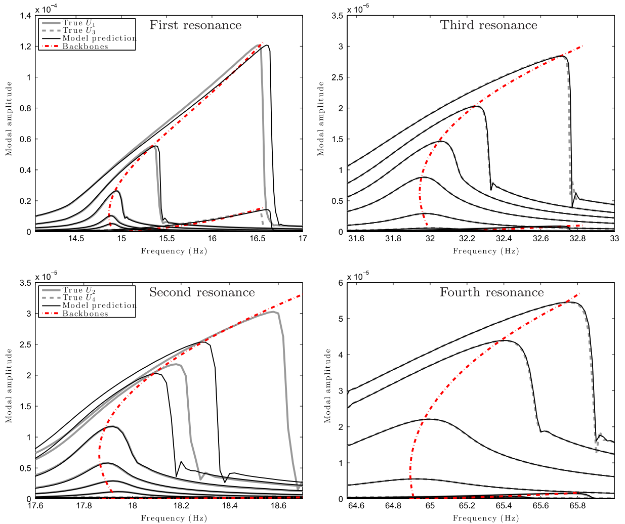
Fig. 8. Sine stepped simulation of the fitted model that considers quadratic and cubic nonlinearities on top of the actual system response.
