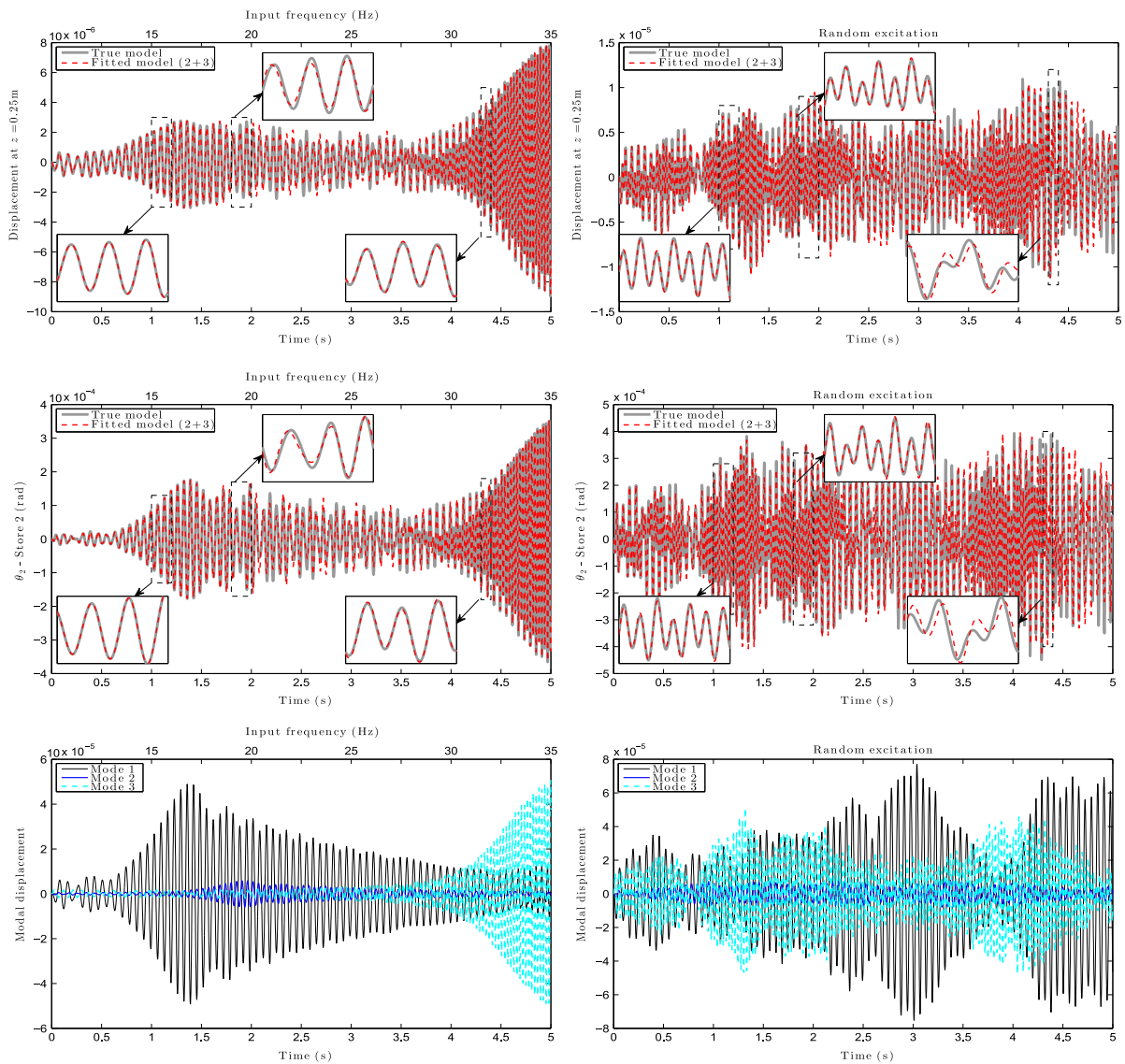
Fig. 9. Vertical displacements of the beam at z=0.25 m (top panels), rotation of one pylon (middle panels) and modal displacements (lower panels) when simulating the response to a sine sweep (left-hand panels) and random (right-hand panels) excitation of the fitted model that considers quadratic and cubic nonlinearities on top of the responses of the true model of the example structure.
