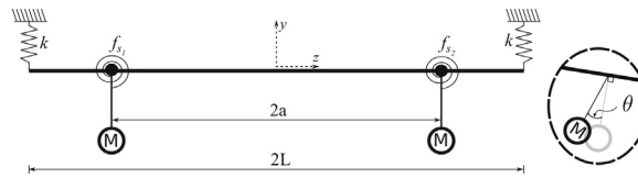
Fig. 2. Example of a wing with stores on pylons connected through nonlinear rotational springs.
