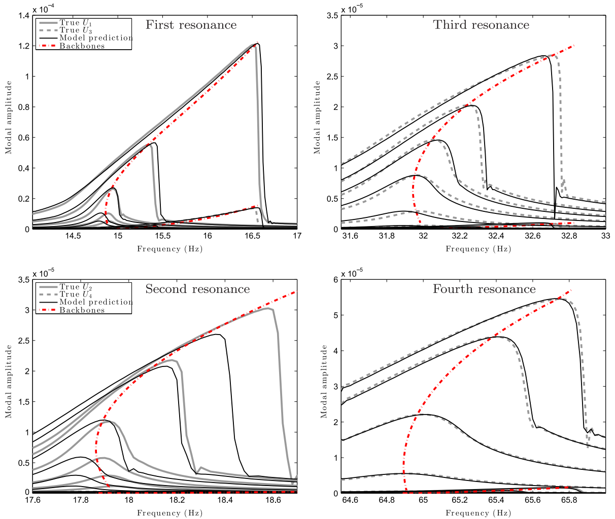
Fig. 7. Sine stepped simulations of the fitted model that considers cubic nonlinearities only on top of the actual system response.
