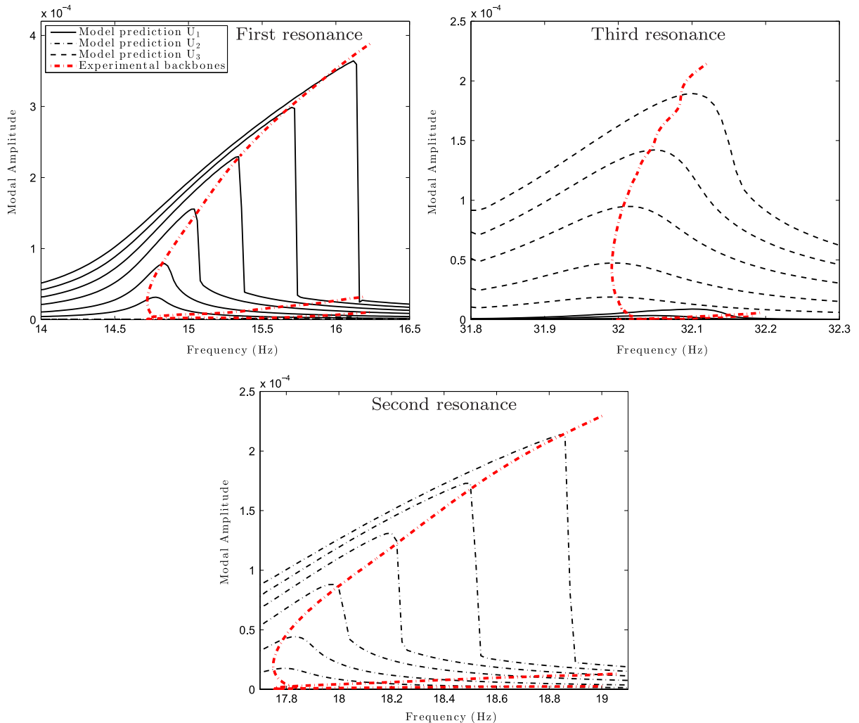
Fig. 15. Sine stepped simulations of the fitted model that considers cubic nonlinearities only on top of the experimental backbone curves of the test structure.
