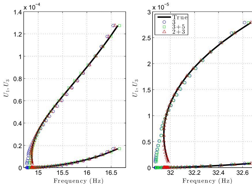
Fig. 5. Best fitting case of the trial nonlinear models on top of the systems backbone curves for the first and third resonances.
