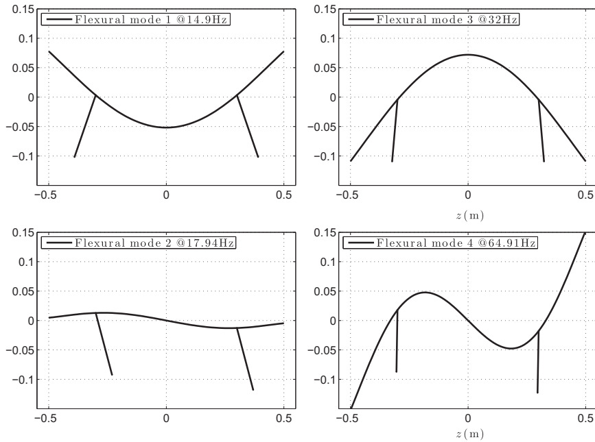
Fig. 3. Schematics for the first four flexural mode shapes of the underlying linear dynamics of the example structure.
