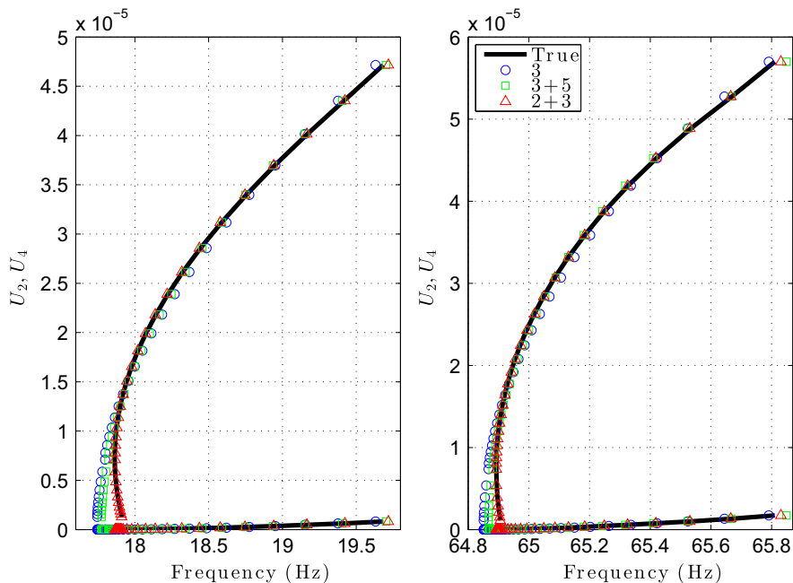
Fig. 6. Best fitting case of the trial nonlinear models on top of the systems backbone curves for the second and fourth resonances.
