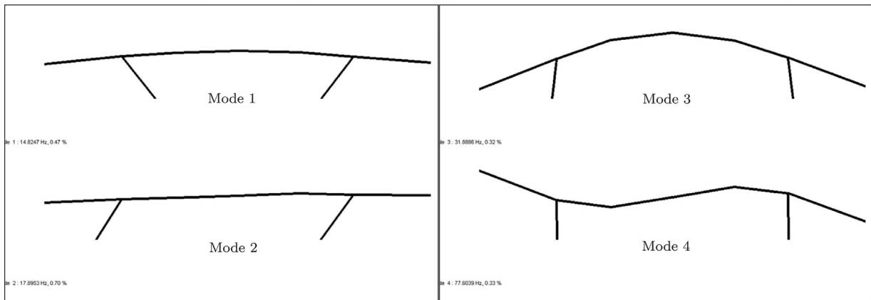
Fig. 12. First four mode shapes of the underlying linear system of the test model.
