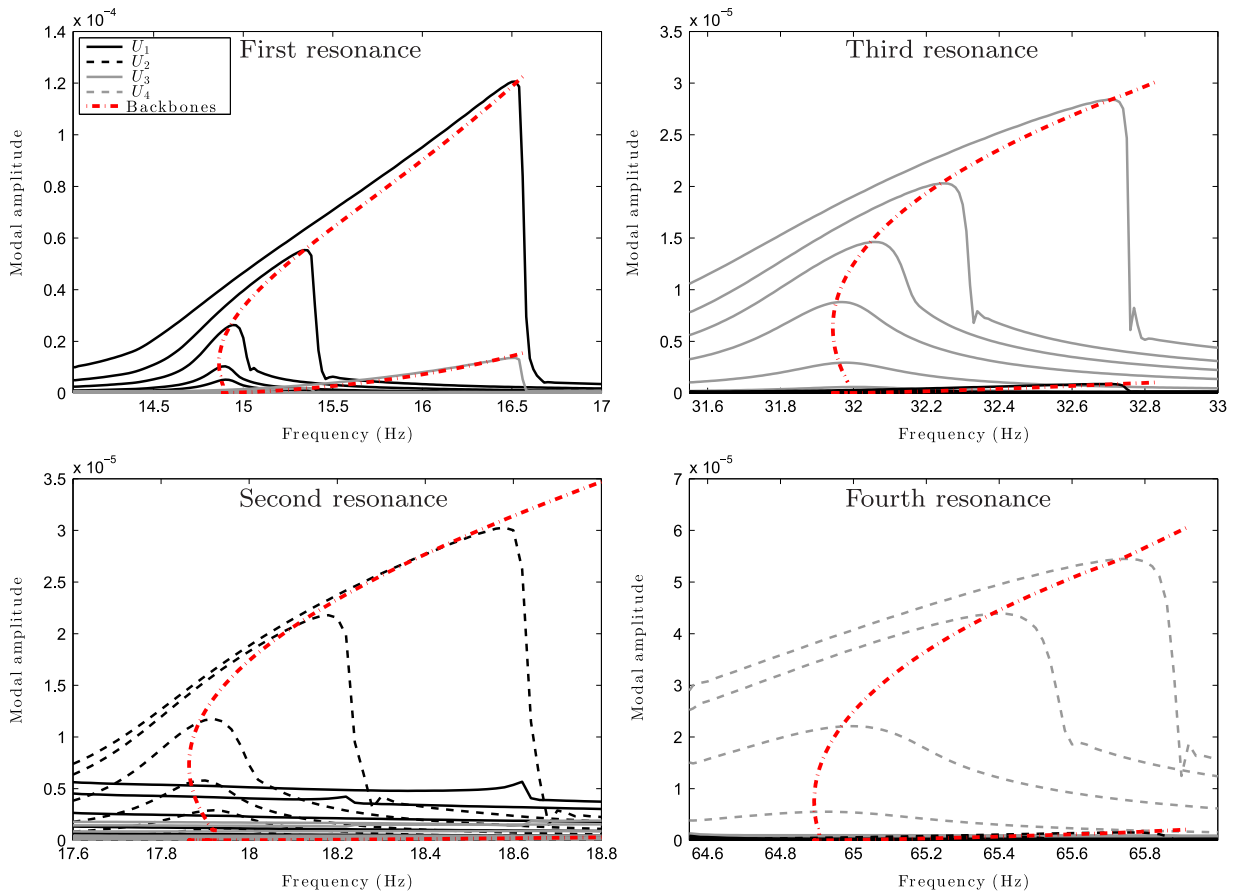
Fig. 4. Backbone curves overlying the stepped sine responses of the example model around the four frequencies of interest. Here U_i is the spectral component of the i -th flexural vibration mode at each frequency in the steady-state.
