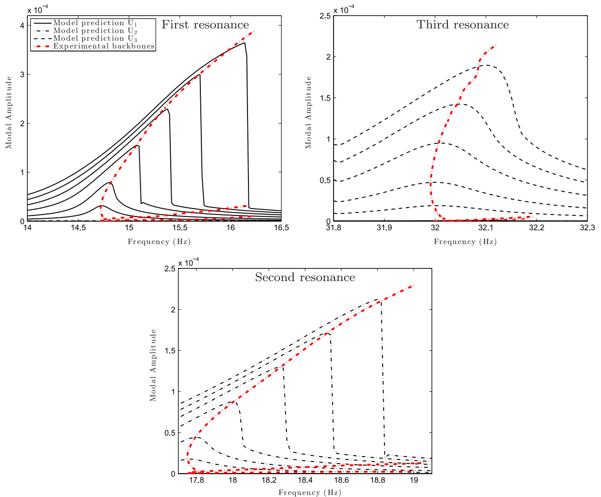
Fig. 16. Sine stepped simulations of the fitted model that considers quadratic, cubic, quartic and quintic nonlinearities on top of the experimental backbone curves of the test structure.
