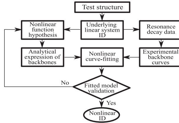
Fig. 1. Diagram of the proposed procedure for the identification of nonlinear systems from backbone curves.
