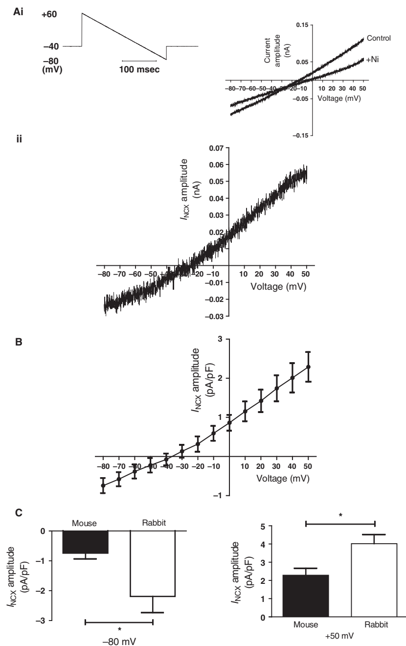
Figure 6. I_{\text{NaCa}} . (Ai) Representative descending voltage ramp protocol (left hand side) used to elicit I_{\text{NaCa}} , and current traces elicited by this protocol (right hand side) in absence (control) and presence of 5 mmol/L \text{Ni}^{2+} (+ Ni). Start to start interval of the protocol was 3 sec. (Aii) Representative current trace of the \text{Ni}^{2+} -sensitive current: I_{\text{NaCa}} (obtained by subtracting the residual current recorded in the presence of \text{Ni}^{2+} from that in control). (B) I - V relationship for \text{Ni}^{2+} -sensitive I_{\text{NaCa}} ( n = 6 ). \text{Ni}^{2+} -sensitive currents were sampled at 10 mV intervals, normalized to current density and pooled. (C) Comparison of the I_{\text{NaCa}} current amplitude measured in mouse ( n = 6 ) and in rabbit ( n = 5 ) atrioventricular nodal cells at -80 and +50 mV. Asterisks denote statistical significance (unpaired t test; P < 0.05 ).
