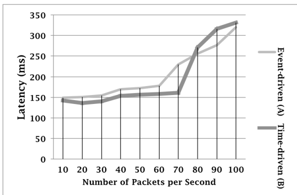
Figure 5: Latencies associated with Event-driven and Time-driven applications delivered to External subscriber via a central node.
