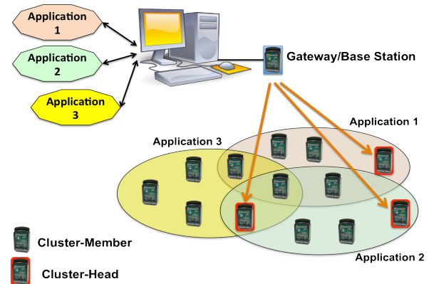
Figure 2: Multiple overlapping clusters for concurrent applications
