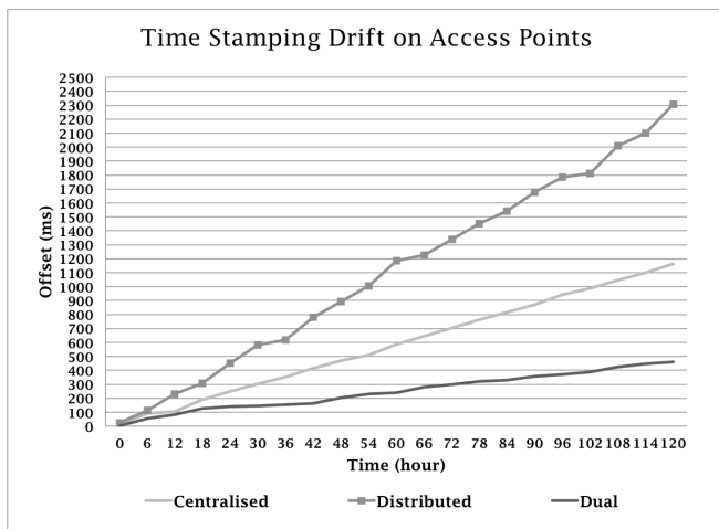
Figure 9: Drift in the time-stamping of the packets using Centralised, Distributed and the Dual modes.
