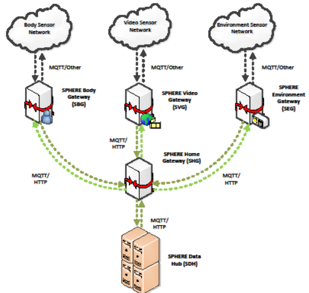
Figure 1: An overview of the SPHERE system architecture.
