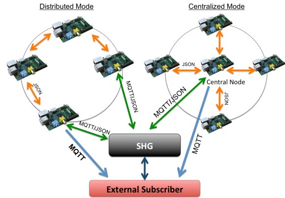
Figure 3: Distributed and Centralised agent-based model.
