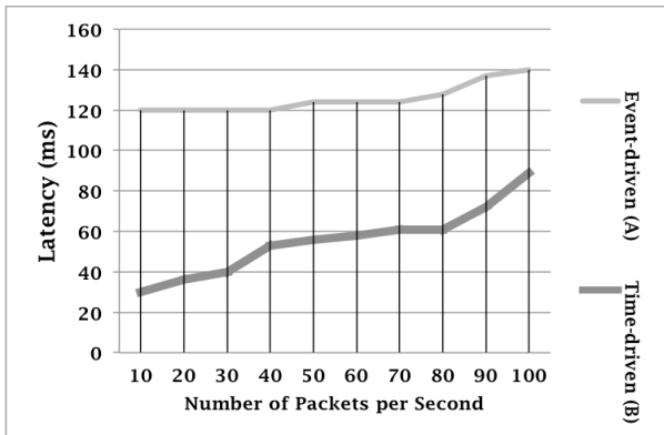
Figure 8: Latencies associated with Event-driven and Time-driven applications delivered to External subscribers via the SHG.
