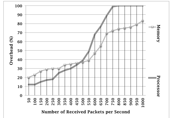
Figure 6: Processor and Memory overheads based on the number of packets received per second.
