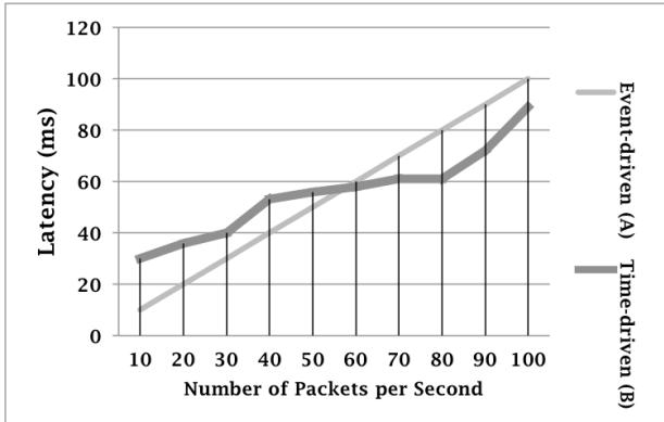
Figure 4: Latencies associated with Event-driven and Time-driven applications delivered to Local subscriber via a central node.
