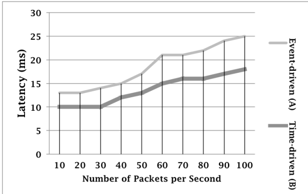
Figure 7: Latencies associated with Event-driven and Time-driven applications delivered to Local subscribers bypassing the SHG
