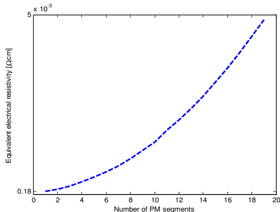
Fig. 10. The equivalent electrical resistivity of the PM material \rho(u) versus number of PM segments
