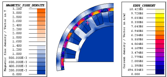
Fig. 4. Distribution of magnetic flux density within the stator and rotor core packs together with vector plot of the eddy-currents in the PM poles from 2D FEA – rated operation, n = 4000\text{rpm} , I_q = 177\text{A}_{\text{rms}}
