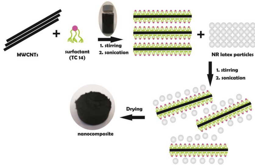
Fig. 1 Schematic of the latex technology
