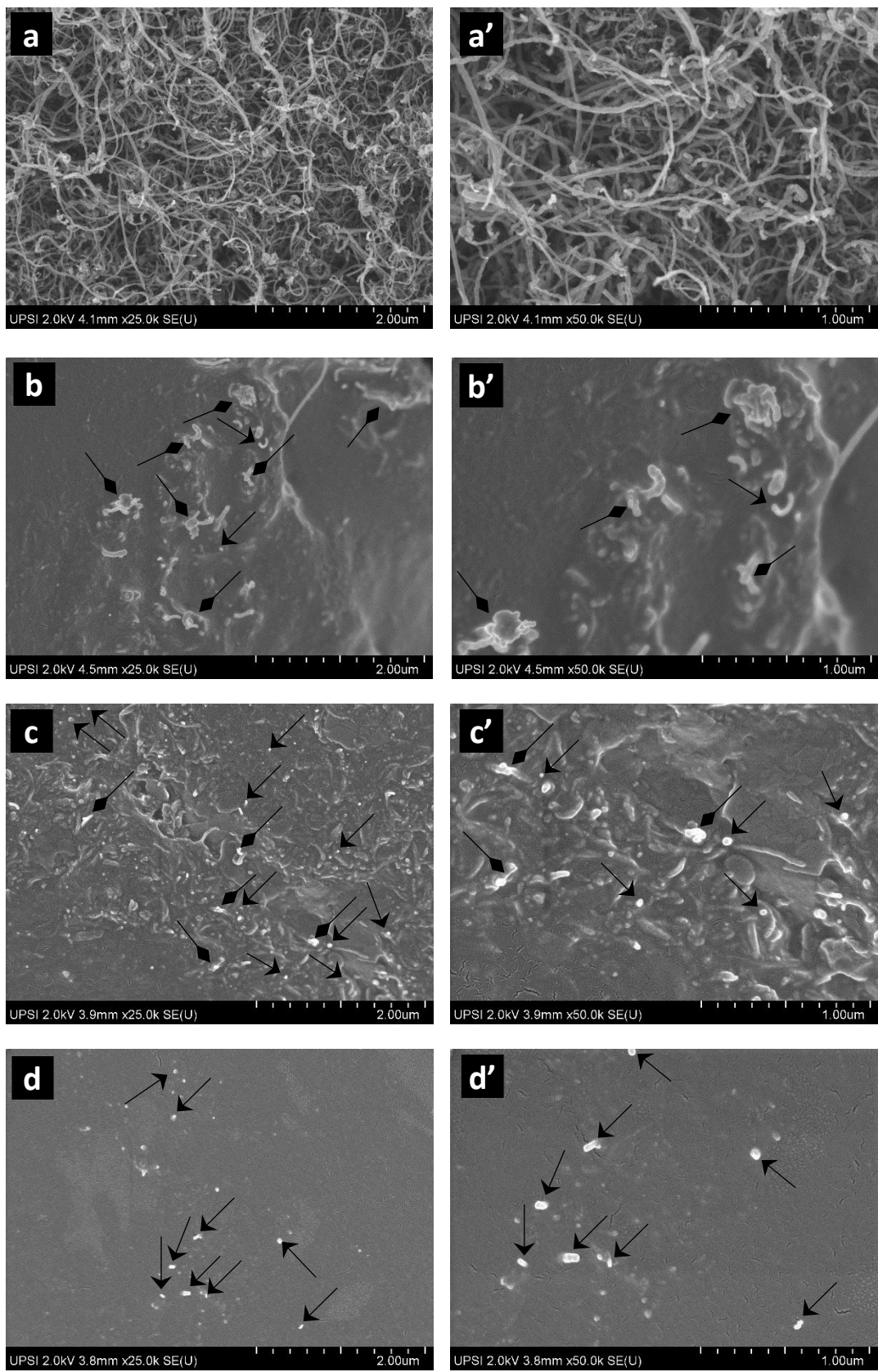
Fig. 3 FESEM images of MWCNTs only (a and a') and MWCNTs/NR-latex: in the absence of surfactant (b and b'); with SDS (c and c'); with TC14 (d and d').
