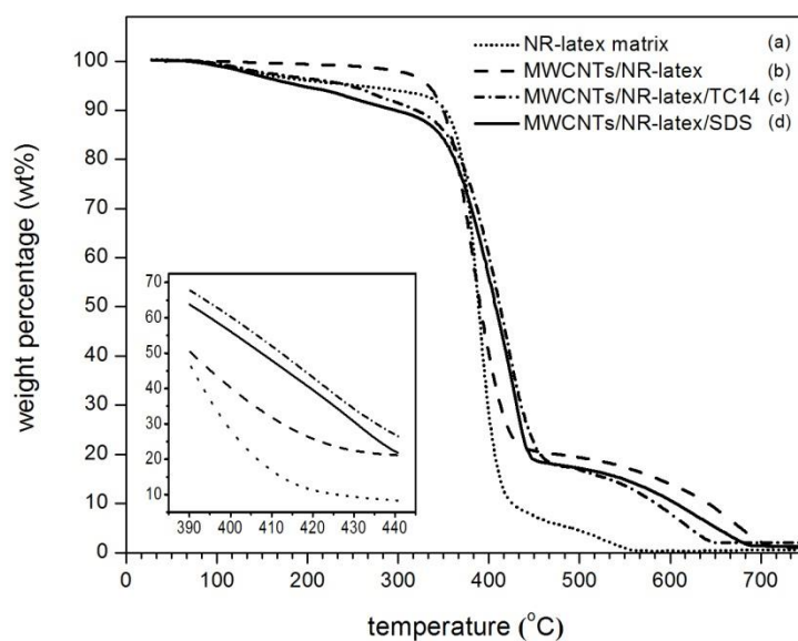
Fig. 5 TGA curves for the (a) NR-latex matrix, (b) MWCNTs/NR-latex, (c) MWCNTs/NR-latex/TC14, and (d) MWCNTs/NR-latex/SDS.
