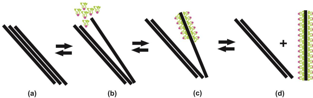
Fig. 7 Stabilisation of individual MWCNTs by a surfactant: (a) MWCNTs bundles; (b) high local shear is formed; (c) the surfactant begins to adsorb onto the MWCNT surface; and (d) the individual MWCNTs stabilised by surfactant are separated from the bundles.
