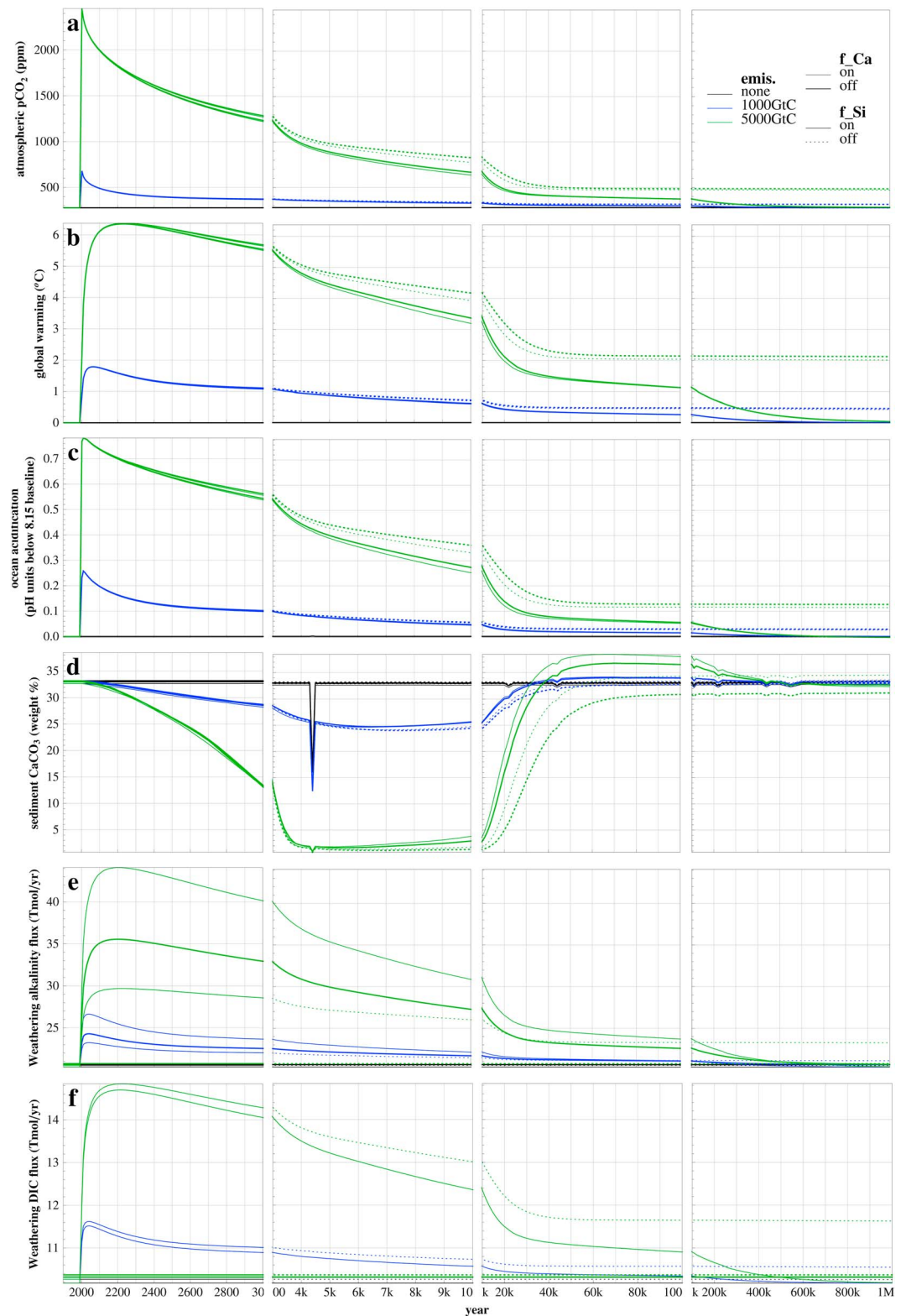
Figure 3. Evolution of (a) atmospheric p\text{CO}_2 , (b) global surface warming, (c) surface ocean acidification, (d) sea floor sedimentary carbonates, (e) weathering alkalinity flux, and (f) weathering DIC flux, over 1 Myr for 1000 PgC (blue) and 5000 PgC (green) emissions pulses versus a control run with no emissions (black), with carbonate and silicate weathering feedbacks (f_Ca and f_Si, respectively) on/off in the global average (0-D) version of the model. Note that the blips in sediment \text{CaCO}_3 are an artifact of the model restart process (model runs were restarted every 4.4 kyr) caused by the sediments taking a few years to “warm up” and output being taken during this time.
