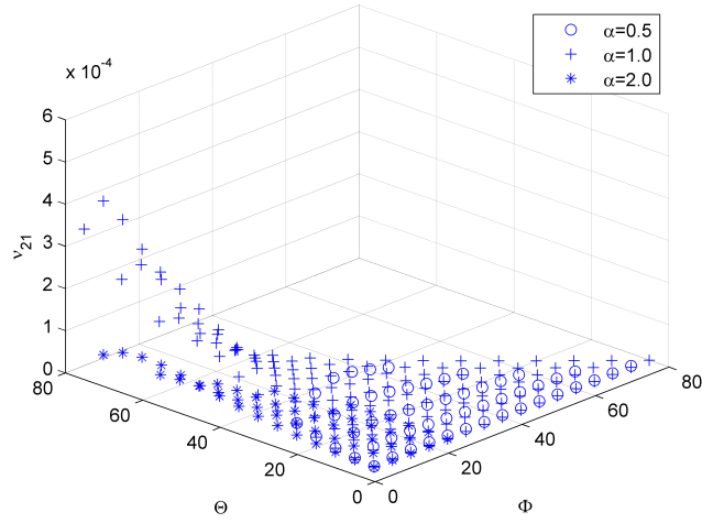
Figure 9 FE homogenization for the Poisson's ratio \nu_{21} vs \phi and \theta for \beta = 0.1, \gamma = 1, \alpha = 0.5, 1.0, 2.0 .
