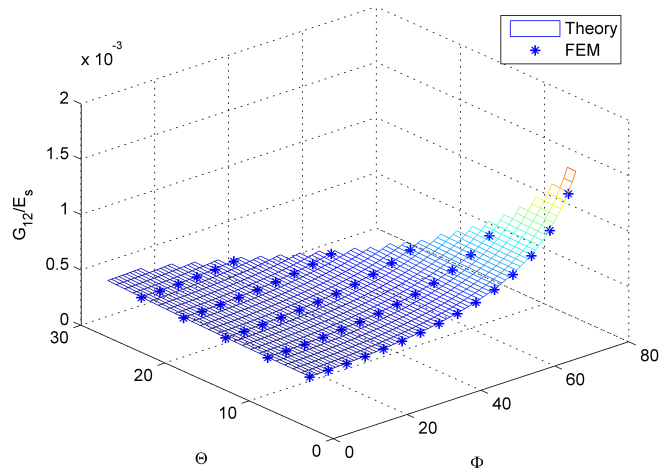
Figure 10 FE homogenization and theoretical predictions for the non-dimensional elastic modulus G_{12}/E_s versus \phi and \theta for \beta = 0.1, \gamma = 1, \alpha = 0.5 .
