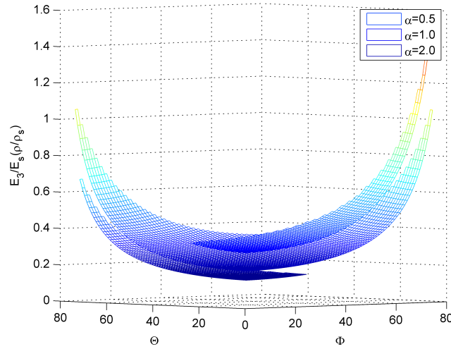
Figure 13 Theoretical results for relative density versus \varphi and \theta for \beta = 0.1, \gamma = 1, \alpha = 0.5, 1.0, 2.0 .
