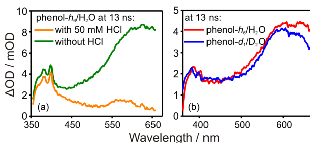
Figure 3. (a) TA spectra of phenol with and without 50 mM HCl (the electron scavenger) measured at t = 13 ns. (b) TA spectra of phenol- h_6 /H 2 O and phenol- d_1 /D 2 O measured at t = 13 ns.
