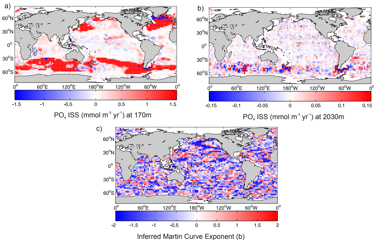
Figure 2. Example of using a GCM transport matrix to estimate \text{PO}_4 remineralisation rates. (a) The estimated \text{PO}_4 remineralisation rates generated using the MITgcm transport matrix at 170 and (b) 2030 m. (c) Power-law flux curve exponents (b) inferred from the estimated remineralisation rates by fitting a linear function to the log-transformed data as in Fig. 1b.
