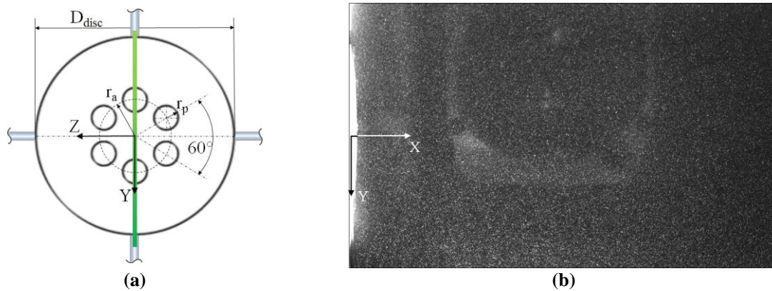
Figure 15 (a) Disc used in the experiment for the PIV analysis. (b) Exemplary PIV image illustrating the reflections off the disc surface
