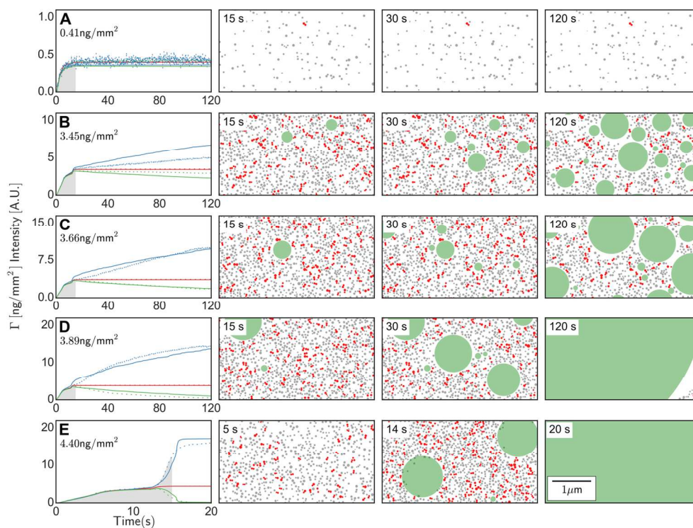
Figure 5 Measurements and simulations of surface loading dependent vesicle rupture and lipid mixing show rupture of clustered vesicles is the rate limiting step for PSB formation: Measured (dashed) and simulated (solid) traces for RIF (red), RhoB (green) and OG488 (blue) for surface loadings of (A) 0.41, (B) 3.45, (C) 3.66, (D) 3.89, and (E) 4.4 \text{ng}\cdot\text{mm}^{-2} . Injection period is marked with a grey background. Images to the right show the spatial distribution of isolated vesicles (grey), vesicles in contact with other vesicles (red) and bilayers (green) at different time points. Scale bar 1\mu\text{m} .
