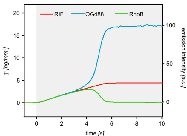
20 21 22 23 24 25 26 27 28 29 30 31 32 33 34 Figure 1 Vesicle binding to silica is diffusion rather than affinity controlled and vesicle rupture and 35 membrane merger begins well before surface saturation: Simultaneous measurement of vesicle 36 deposition (RIF trace, red), vesicle rupture (Oregon Green 488, blue) and membrane merger 37 (Sulforhodamine, green). Injection period is marked with a grey background. 38 39 40 41 42
