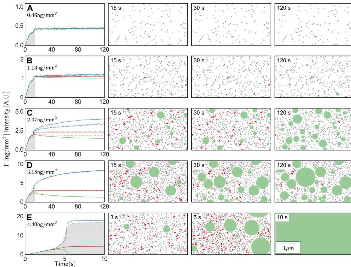
Figure 3 Measurements and simulations of surface loading dependent vesicle rupture and lipid mixing show rupture of clustered vesicles is the rate limiting step for SSB formation: Measured (dashed) and simulated (solid) RIF (red), RhoB (green) and OG488 (blue) traces for surface loadings of (A) 0.46, (B) 1.13, (C) 2.37, (D) 3.18, and (E) 4.4 \text{ng}\cdot\text{mm}^{-2} . Injection period is marked with a grey background. Images to the right show the simulated spatial distribution of isolated vesicles (grey), vesicles in contact with other vesicles (red) and bilayers (green) at different time points for the corresponding simulated fluorescence traces.
