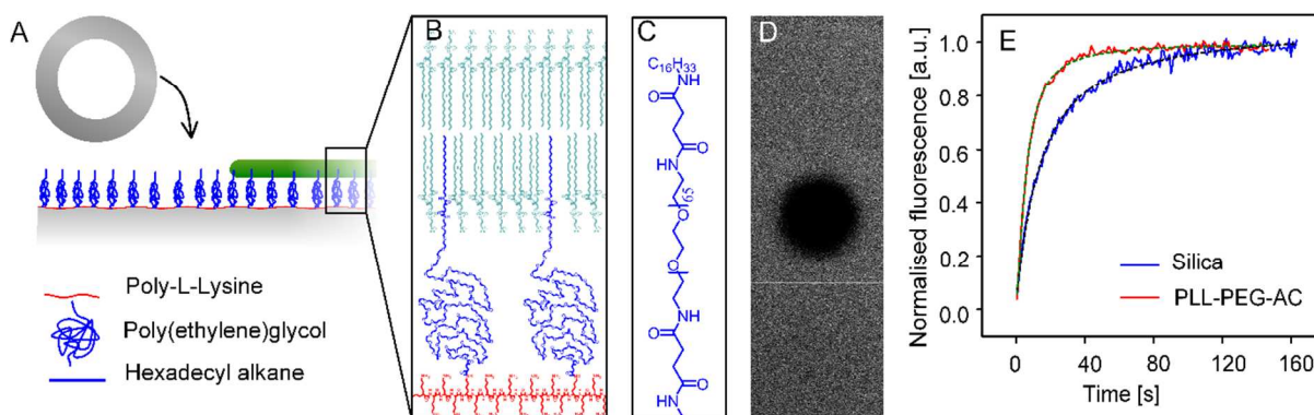
45 46 47 48 49 50 51 52 53 54 55 56 57 58 59 60 Figure 4 Vesicle deposition on PLL-PEG-AC leads to bilayer formation: (A) Surface architecture of silica coated with PLL-PEG-AC. (B) Chemical architecture of PLL-PEG-AC and SOPC bilayer (C) Chemical structure of PEG-AC attached to PLL. (D) Confocal laser scanning images showing fluorescence-recovery after photo-bleaching for a bilayer formed by SOPC vesicle doped with 0.2% OG488-DHPE on PLL-PEG-AC; first frame: immediately before photo-bleaching, second frame: immediately after photobleaching, third frame: 30 s post bleaching. (E) Normalised fluorescence from the bleached region demonstrating efficient recovery over time for silica (blue line) and PLL-PEG-AC (red line).
