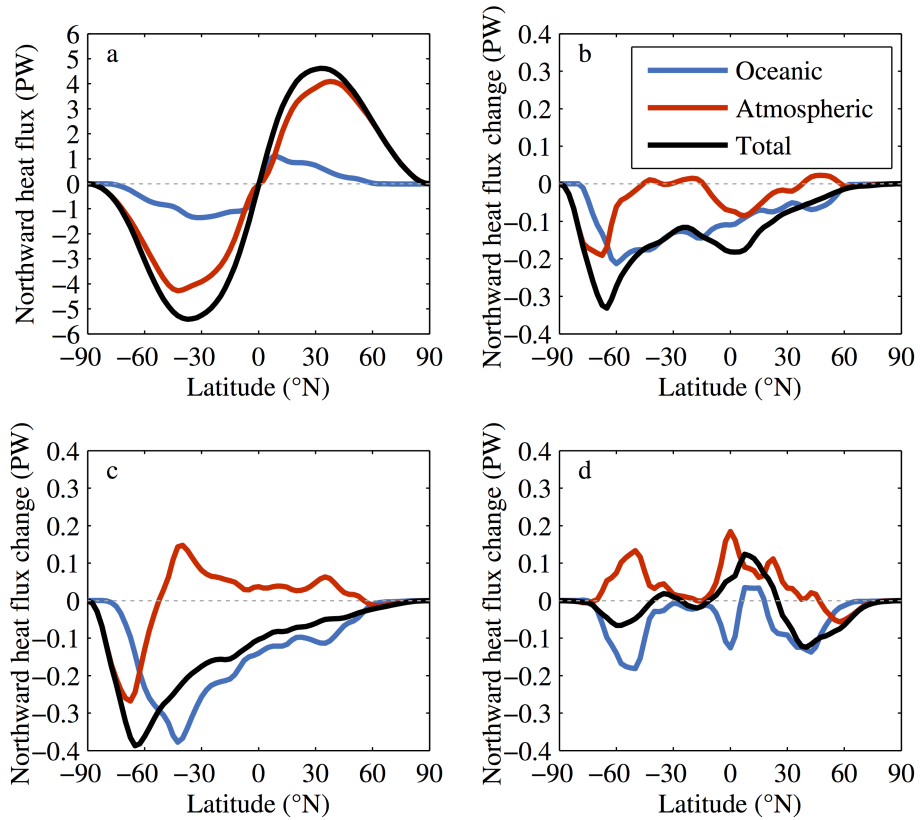
Figure 7: General form of the global meridional (northward) heat flux (PW), shown for the unglaci­ated Rupelian (a). Changes in the northward heat flux in response to glaci­ation are shown for the Priabonian (b) and Rupelian (c), and changes in response to gateway opening (unglaci­ated Rupelian – unglaci­ated Priabonian) are shown in (d). In all figures, black lines show total, red lines show atmospheric and blue lines show oceanic heat fluxes.
