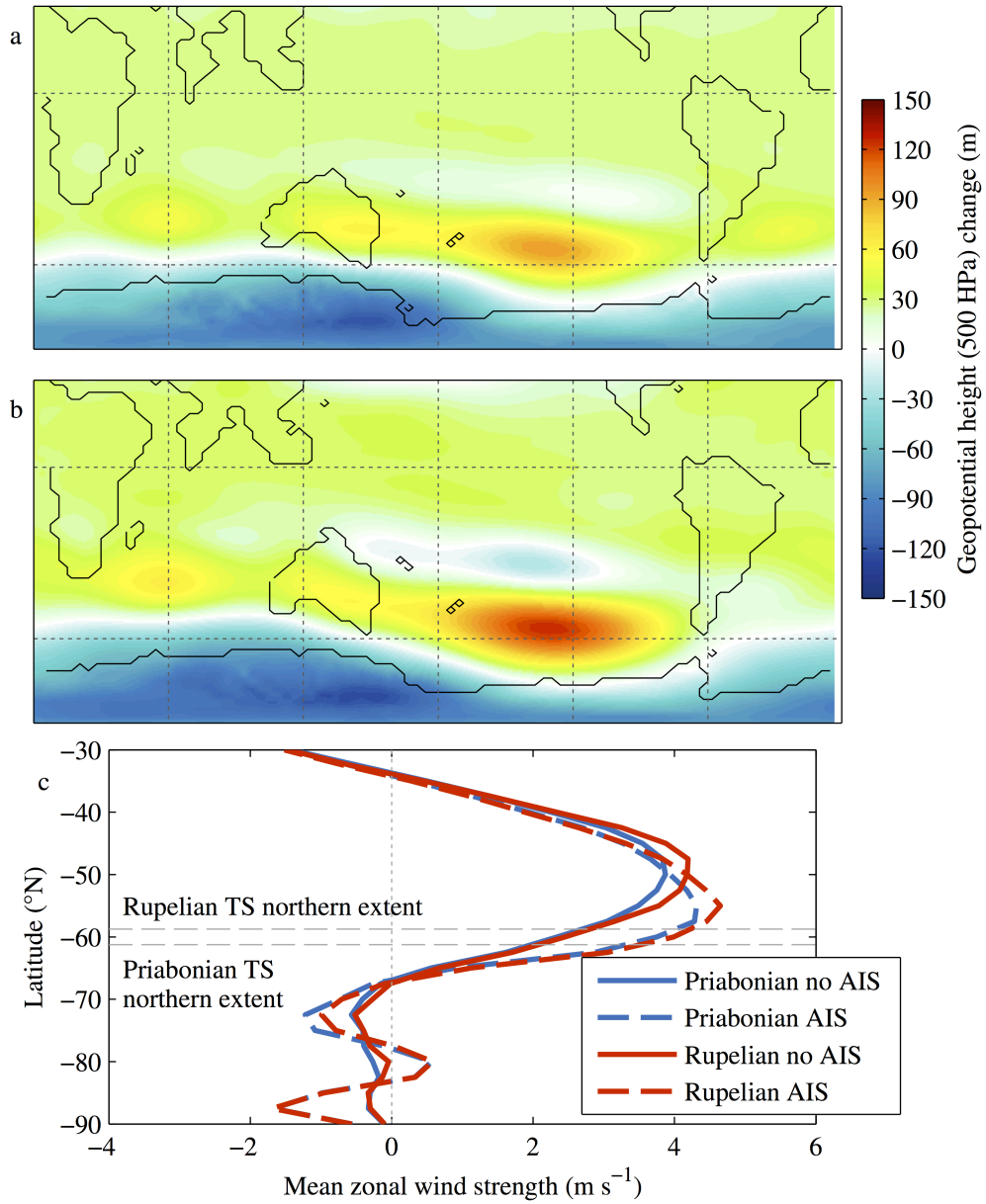
Figure 4: Changes in annual mean 500 hPa geopotential height (m) in response to Antarctic glaciation for the Priabonian (a) and Rupelian (b), and mean zonal westerly wind strength ( \text{m s}^{-1} ) for each stage and ice sheet configuration (c).
