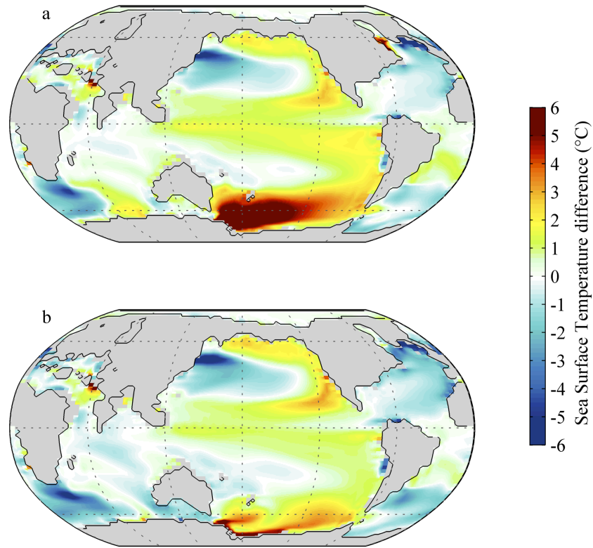
Figure S4: Sea surface temperature difference between the stages for the same ice sheet configuration ( ^{\circ}\text{C} ), shown for the unglaciated Rupelian – unglaciated Priabonian (a) and the glaciated Rupelian – glaciated Priabonian (b).
