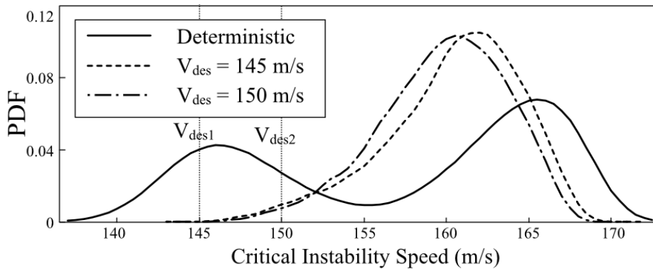
Figure 8: Comparison of instability speed PDFs for different optimised stacking sequences with potential ply orientations at 5^\circ increments
