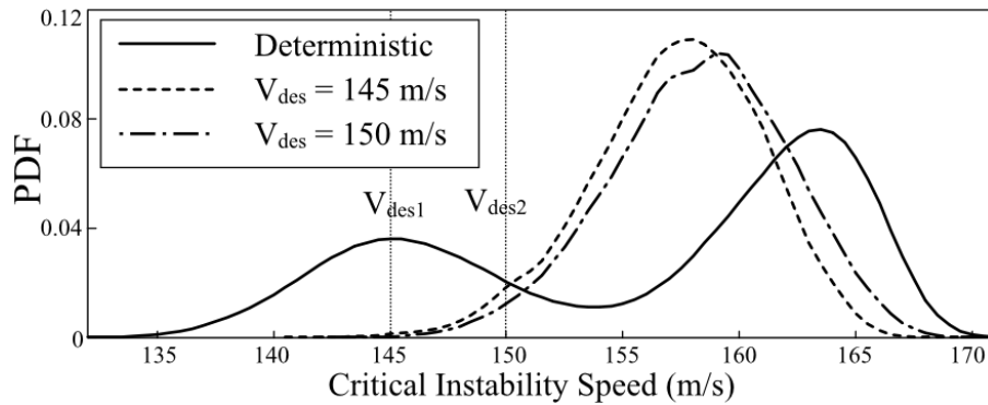
Figure 7: Comparison of instability speed PDFs for different optimised stacking sequences with 0^\circ , \pm 30^\circ , \pm 45^\circ , \pm 60^\circ and 90^\circ plies
