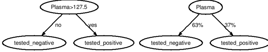
Fig. 1: Two types of models; on the left is the model using a fixed threshold while on the right is the model using percentiles. For each deployment context, the decision tree is deployed in such a way that the deployment instances are split to the leaves in the same percentile amounts of 63% and 37%.
