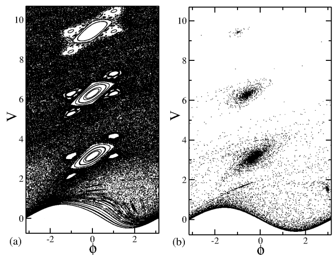
FIG. 1. Comparison between phase space for conservative and dissipative dynamics. In (a) \varepsilon = 0.6 and \gamma = 1.0 , and in (b) \varepsilon = 0.6 and \gamma = 0.9 . In (b) the thick black regions are the sinks and the bottom attractor. Also, all the spread dots are the transient.
