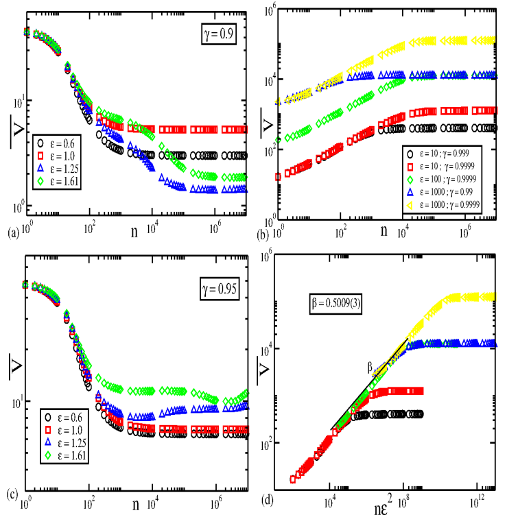
FIG. 2. Color online: Behaviour of the average velocity curves for an extensive range of \epsilon and \gamma . In (a) and (c), we have a high dissipation and low \epsilon , and the dynamics are basically controlled by the attracting fixed points. In (b) and (d), we have small dissipation and high \epsilon . Here the dynamics is ruled by the attractor localized in the bottom, embedded with the vibrating wall. Also, in (d) a rearrange in the horizontal axis is made, in order to make all the curves start to grow together. This rearrange is convenient, when we make use of the scaling techniques.
