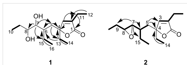
Figure 2: COSY connectivities (bold bonds) and selected HMBC (arrows) correlations for plakilactones G ( 1 ) and H ( 2 ).
