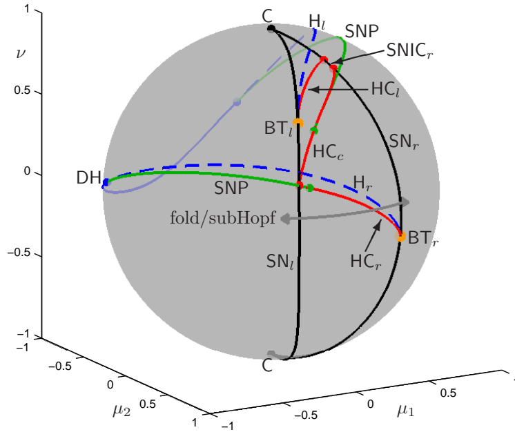
Figure 2: Bifurcation diagram of system (3) with b = 0.75 on the unit sphere in (\mu_1, \mu_2, \nu) -space. Color in on-line version: red, homoclinic (HC); blue, Hopf bifurcation (H; solid: supercritical, dashed: subcritical); black, saddle-node (SN); orange, Bogdanov–Takens point (BT); green, saddle node of periodics (SNP); degenerate Hopf and cusp are labeled DH and C, respectively. A path of pseudo-plateau bursting is indicated; we used the circle segment on the unit sphere with \nu = 0.1 and \mu_1 = \sqrt{1 - \nu^2} \cos(2\pi\vartheta) , where \vartheta varies between 0.245 \pm 0.065 .
