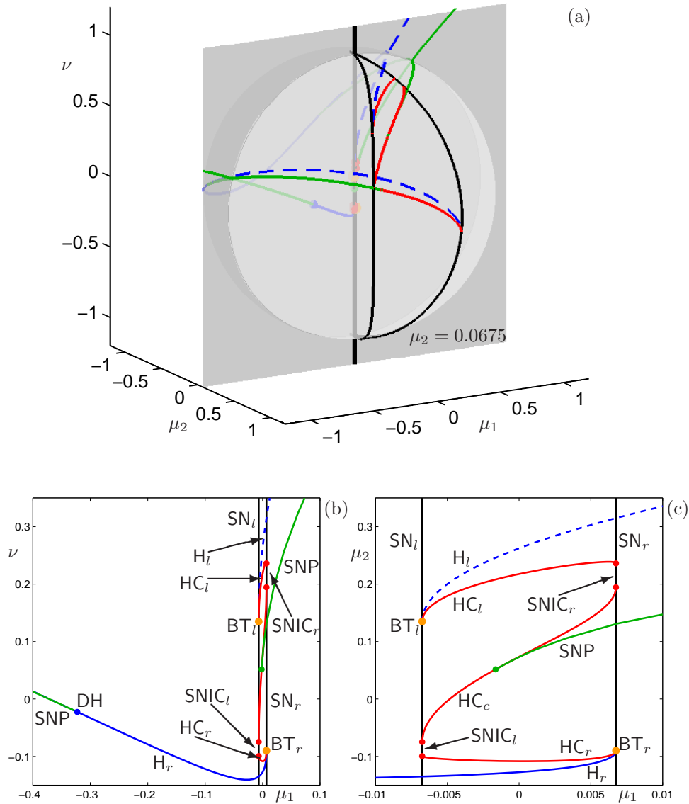
Figure 3: Bifurcation diagram of (3) with b = 0.75 and \mu_2 = 0.0675 ; the bifurcation diagram on the unit sphere with b = 0.75 from Figure 2 is shown for reference in panel (a) with the (\mu_1, \nu) -plane shown in panel (b) and an enlargement in panel (c). Colors and symbols as in Figure 2.
