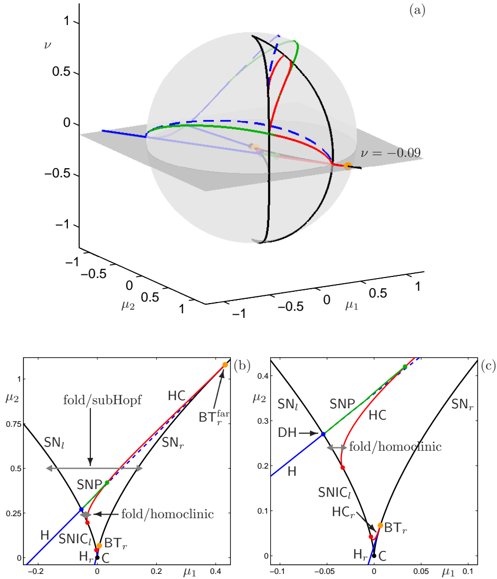
Figure 4: Bifurcation diagram of (3) with b = 0.75 and \nu = -0.09 ; the bifurcation diagram on the unit sphere with b = 0.75 from Figure 2 is shown for reference in panel (a) with the (\mu_1, \mu_2) -plane shown in panel (b) and an enlargement in panel (c). Note that there are two Bogdanov–Takens points, BT_r and BT_r^{\text{far}} , on the same side SN_r of the cusp point C ; the point BT_r is also contained in the \mu_2 -slice shown in Figure 3. Two burst paths are indicated, which are the fold/subHopf and fold/homoclinic bursters illustrated in Figure 5. Colors and symbols as in Figure 2.
