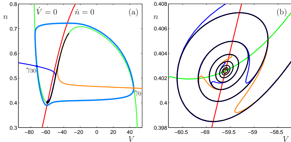
FIG. 8. The isochrons \mathcal{I}(\gamma_0) (orange) and \mathcal{I}(\gamma_{30}) (blue) of the reduced Hodgkin-Huxley equations (4.1) together with the orbit segment \widehat{\mathbf{x}}^r (black) that contains the repelling slow manifold S_\varepsilon^r . Panel (a) shows the isochrons and \widehat{\mathbf{x}}^r in the phase plane and panel (b) shows an enlargement near the equilibrium \mathbf{x}^* (not labeled).
