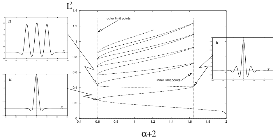
Figure 4: Continuation in \alpha of the one-bump homoclinic orbit from the reversible-Hopf bifurcation at \alpha = 0 of (6) with \delta = 1 and \beta = 0.29 . The ordinate of this and subsequent graphs is a scaling of the vector L_2 -norm of the solution (u(x), u'(x), u''(x), u'''(x))
