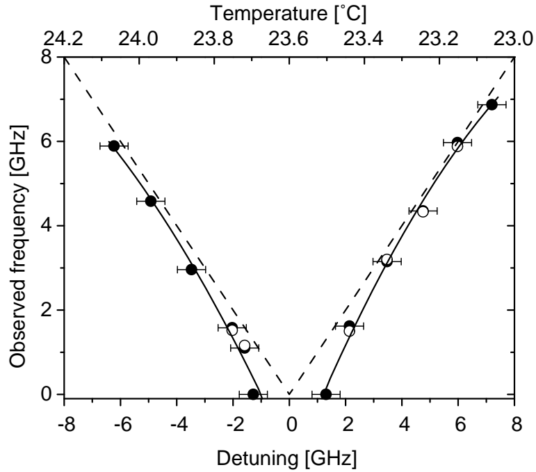
Figure 5. Experimentally observed detuning scenario. The observed frequency of the intensity oscillations is plotted as a function of the detuning. The axis at the top shows the temperature of the heat sink; the dashed line indicates the position of the detuning frequency. Filled circles correspond to laser 1 and open circles to laser 2; the solid curve is an interpolation. A locking region around zero detuning is found. The frequency of the intensity oscillations approach the detuning frequency for large values of detuning.
