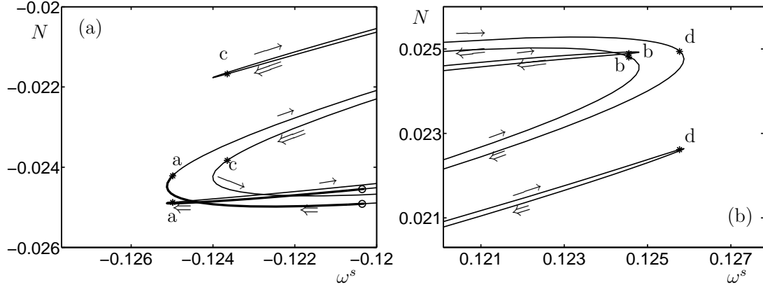
Figure 3. Enlarged view of the (\omega^s, N) -plane for \Delta = 2.5 \times 10^{-3} of the low-inversion region (a) and the high-inversion region (b); compare Fig. 1(d) and (f). The letters ‘a,b,c,d’ label the saddle-node bifurcations; the arrows define the direction of traveling along the branch as in Fig. 2.
