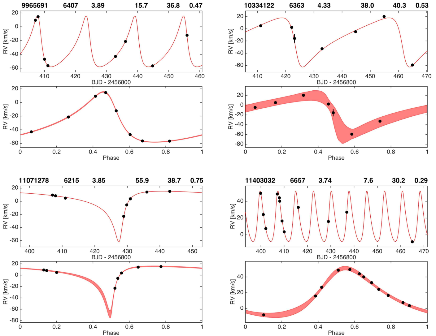
Figure 4. Similar to Figure 1 for KID 9965691, KID 10334122, KID 11071278, KID 11403032. The title for each plot lists (from left to right) KIC ID, T_{\text{eff}} (K), \log g , P (days), K ( \text{km s}^{-1} ), and e .
