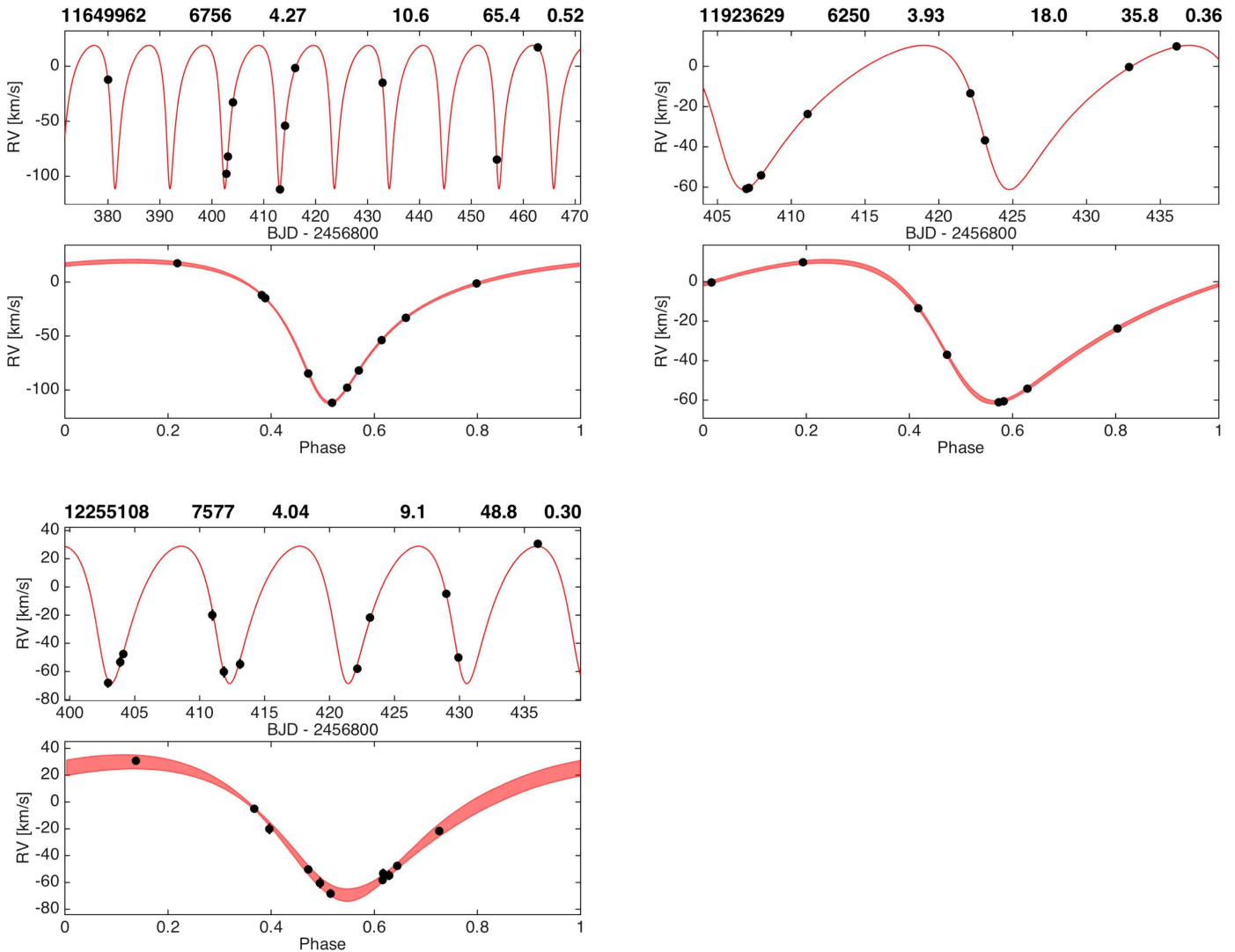
Figure 5. Similar to Figure 1 for KID 11649962, KID 11923629, and KID 12255108. The title for each plot lists (from left to right) KIC ID, T_{\text{eff}} (K), \log g , P (days), K (km s ^{-1} ), and e .
