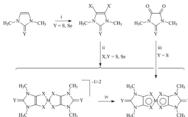
Scheme 1 Synthetic pathway for the preparation of complexes 1–8 . (i) THF, –10 °C, LDA, S/Se; (ii) THF, NiCl 2 ·6H 2 O/K 2 PtCl 4 , Et 4 NI; (iii) refluxing toluene, Lawesson's reagent, Ni powder or PtCl 2 , EtOH after concentration; and (iv) CH 2 Cl 2 , r.t., I 2 . See the ESI† for details.
