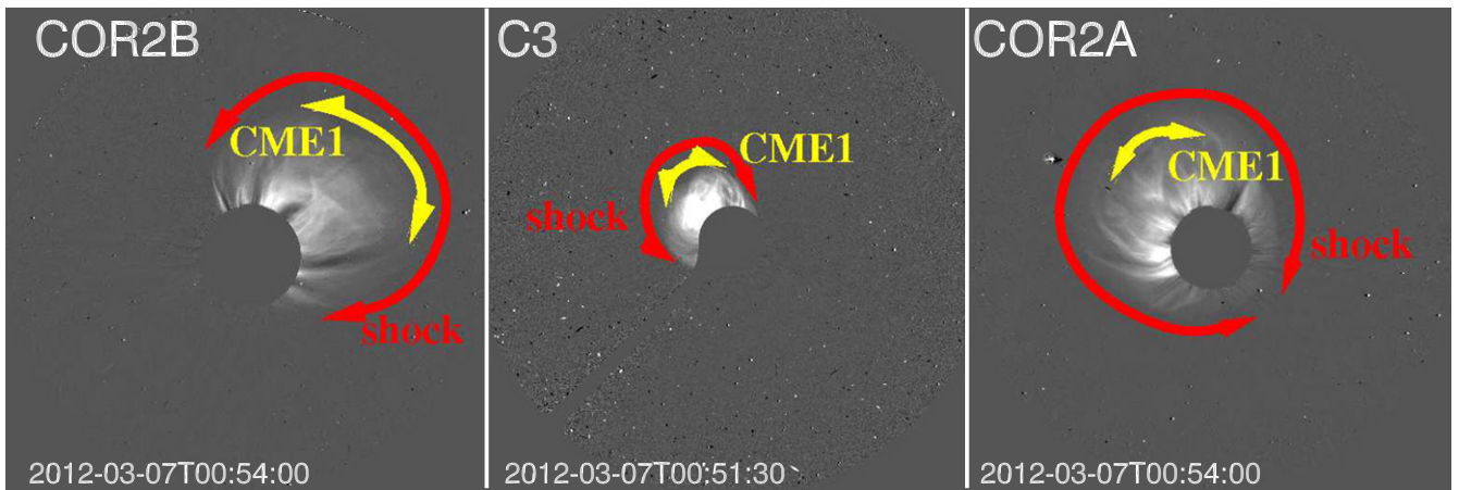
Figure 4. Triple-spacecraft views of CME1 and its associated shock as observed by COR2 on STB (left panel), C3 on LASC0 (middle panel), and COR2 on STA (right panel). The yellow and red double arrows demarcate the extents of CME1 and shock1, respectively.
