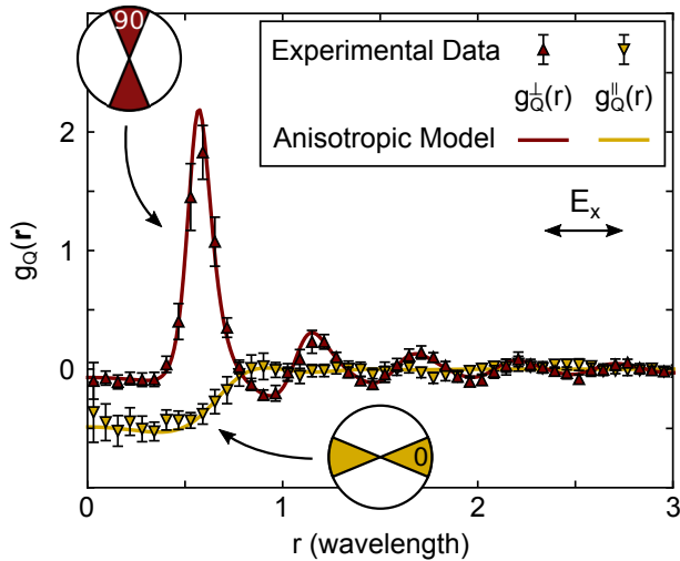
FIG. 4. Directional charge correlation function. We report the two illustrative cases of direction perpendicular (red) or parallel (yellow) to the direction of the considered field component ( E_x ). The distribution function strongly depends on the direction in the plane. Experimental data is represented by the triangles, while lines show our modified model for anisotropic random waves, which perfectly fits the data.
