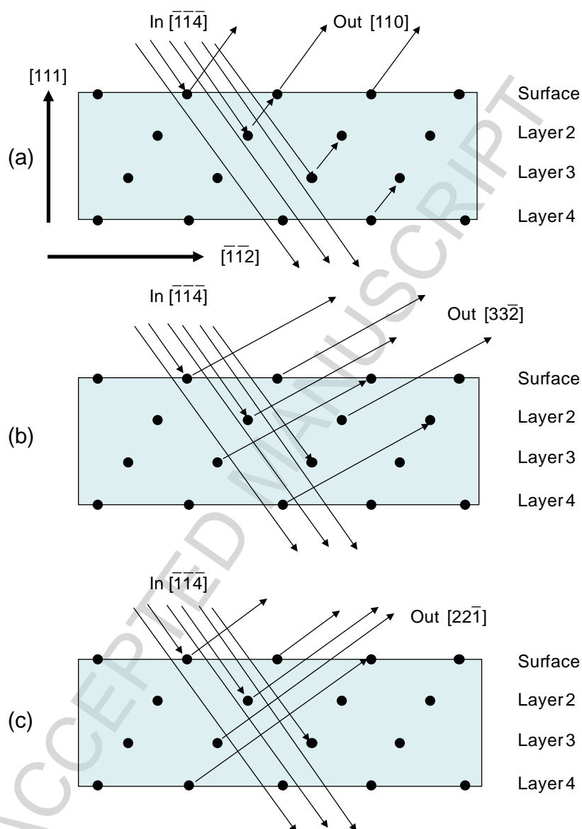
Figure 3: Schematic diagrams showing the ion beam trajectories utilised to achieve (a) 1-, (b) 2- and (c) 3-layer geometries in the azimuth of the fcc \{111\} surface. The arrows represent ion trajectories and show, for example, how the 1st, 2nd and 3rd layer atoms are visible to the incident beam while, by contrast, the 4th layer atoms are shadowed. Similarly, outgoing trajectories show how the phenomenon of blocking can be utilised to achieve layer specific information.
