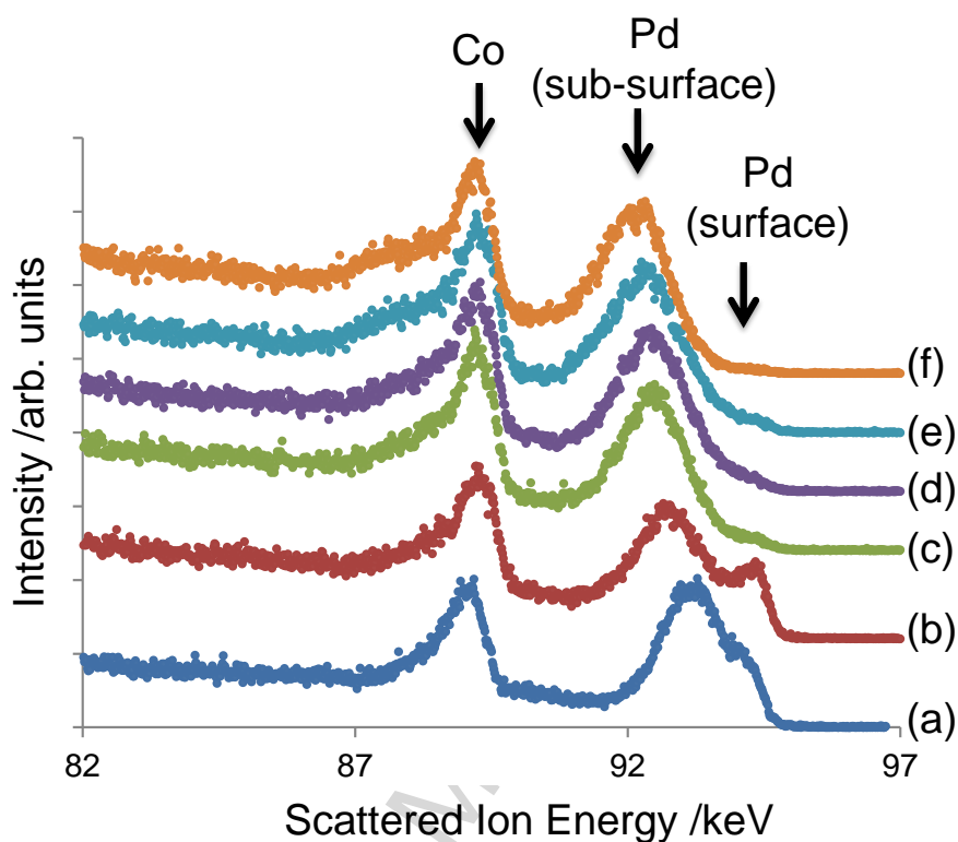
Figure 5: Scattered ion intensity as a function of ion energy in the 2-layer geometry of clean Pd{111} for a 6 ML Co film on Pd{111} (a) as deposited at 300 K; (b) annealed to 560 K; (c) after exposure to 1000 L at 10^{-7} mbar CO; (d) after exposure to 1000 L at 10^{-6} mbar CO; (e) after exposure to 1000 L at 10^{-5} mbar CO; (f) after exposure to 1000 L at 10^{-4} mbar CO. All CO exposures were carried out at 300 K.
