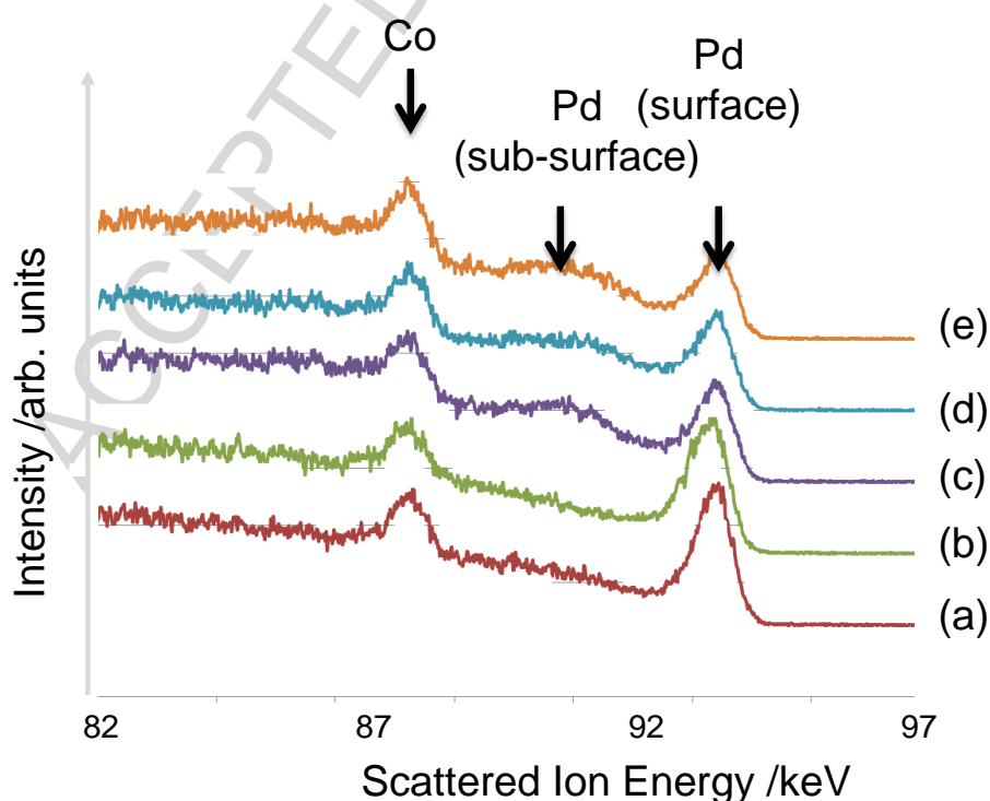
Figure 6: Scattered ion intensity as a function of ion energy in the 2-layer geometry of clean Pd{111} for a 6 ML Co film on Pd{111} (a) annealed to 700 K; (b) after exposure to 1000 L at 10^{-7} mbar CO; (c) after exposure to 1000 L at 10^{-6} mbar CO; (d) after exposure to 1000 L at
