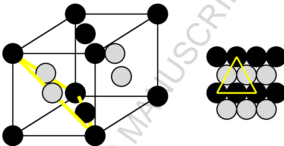
Figure 2: Schematic diagram showing the bulk and {111} surface termination of the ordered CoPd alloy. [20]
