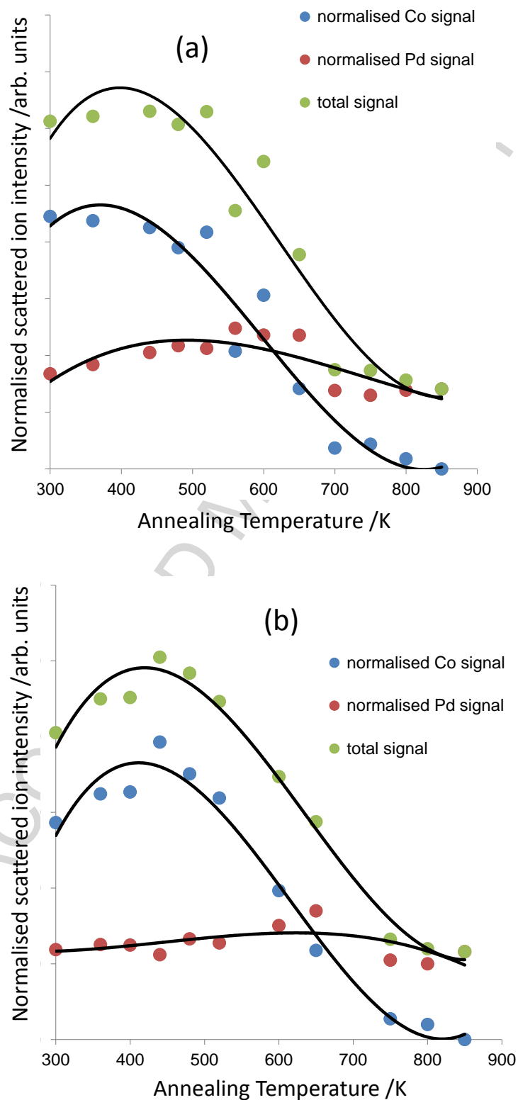
Figure 4: Scattered ion intensity in the (a) 1-layer and (b) 2-layer geometry of the clean Pd{111} surface. The intensity of the Co and Pd peaks were measured separately and then normalised to take into account the dependence of the scattering cross section on the square of the atomic number.
