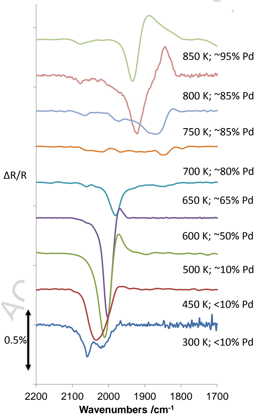
Figure 1b: RAIR spectra as a function of annealing temperature for a 4 ML Co film on Pd{111} deposited at 300 K. Spectra were acquired after exposure to 1000 L CO at a pressure of 10^{-7} mbar with the sample held at 300 K.
