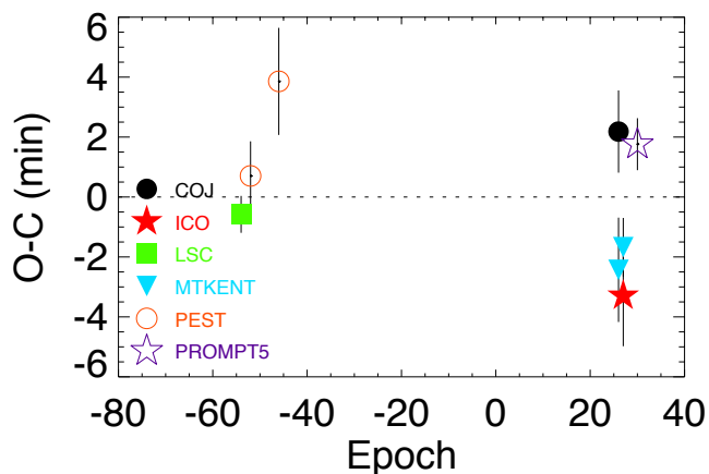
Figure 10. Residuals of the transit times from the best-fit ephemeris. The transit times are given in Table 7. The observatory/telescope abbreviations are the same as in Figure 2. (A colour version of this figure is available in the online journal.)
