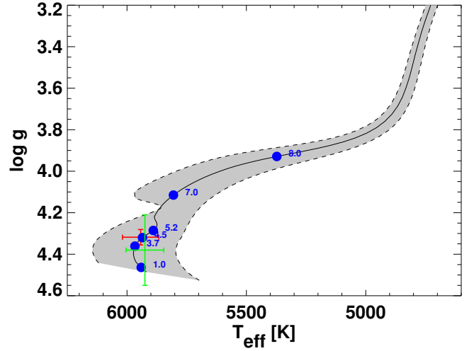
Figure 9. Theoretical H-R diagrams based on Yonsei-Yale stellar evolution models (Demarque et al. 2004). The grey swaths represent the evolutionary track for the best-fit values of the mass and metallicity of the host star from the global fits corresponding to Table 5. The tracks for the extreme range of 1\sigma uncertainties on M_* and [\text{Fe}/\text{H}] are shown as dashed lines bracketing each grey swath. The red cross is the position of KELT-10 using the values obtained from the best fitting global model and the blue points label various ages along the evolutionary track. The green cross is the position of KELT-10 using only the spectroscopically determined \log g_* . (A colour version of this figure is available in the online journal.)
