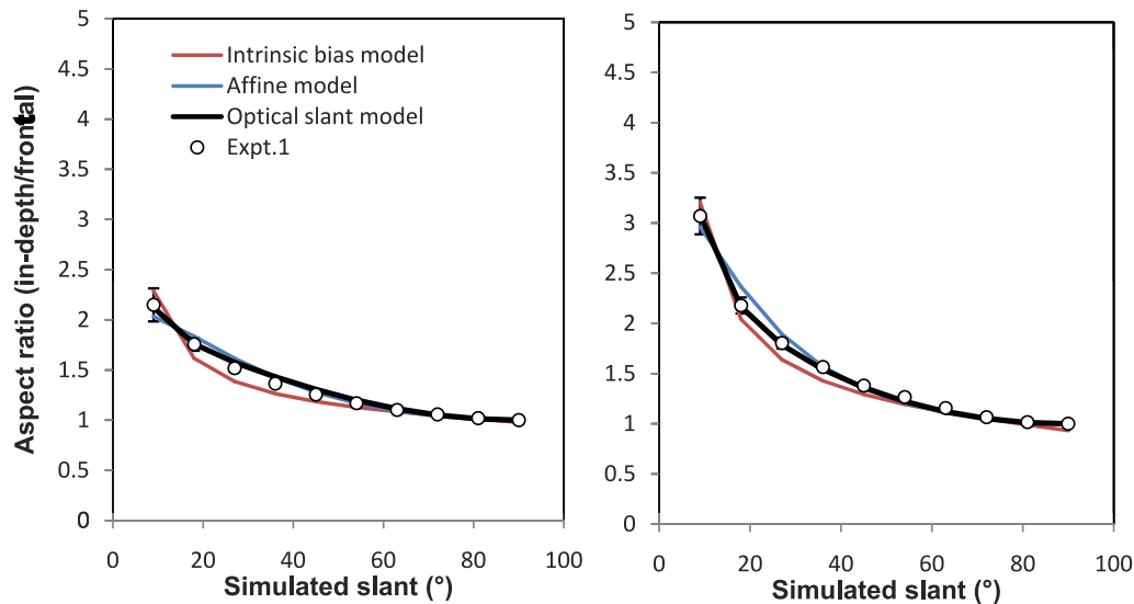
Figure 5. Observed aspect ratio data of Experiment 1 (open circles) and the best fits of the three theoretical models (intrinsic bias model—red lines, affine model—blue lines, and the new optical slant model—black lines) for the 2 m (left panel) and 8 m (right panel) distances, respectively. The parameter values and the sum of squared error (SSE) of the best model fit at the two distances are: \eta = 11.968^\circ ( SSE = 0.0741 ), c = 0.472 ( SSE = 0.0340 ), k = 7.764 ( SSE = 0.0121 ) for the 2 m fit, and \eta = 21.114^\circ ( SSE = 0.1033 ), c = 0.303 ( SSE = 0.0623 ), k = 7.191 ( SSE = 0.0052 ) for the 8 m fit.
