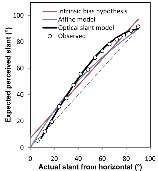
Figure 2. The best model fits to previously observed slant estimation data (open circles). The red line is the best fit for the intrinsic bias model, assuming a constant slant error of 7.2^\circ (sum of squared errors, SSE = 407.66 ). The blue line is the best fit of the affine model based on mis-scaling of binocular disparity, assuming a distance compression ratio of 0.69 ( SSE = 248.61 ). The black line is the best fit of Equation 3, assuming the viewing distance is 0.5 m and k = 10.8 ( SSE = 30.64 ).
