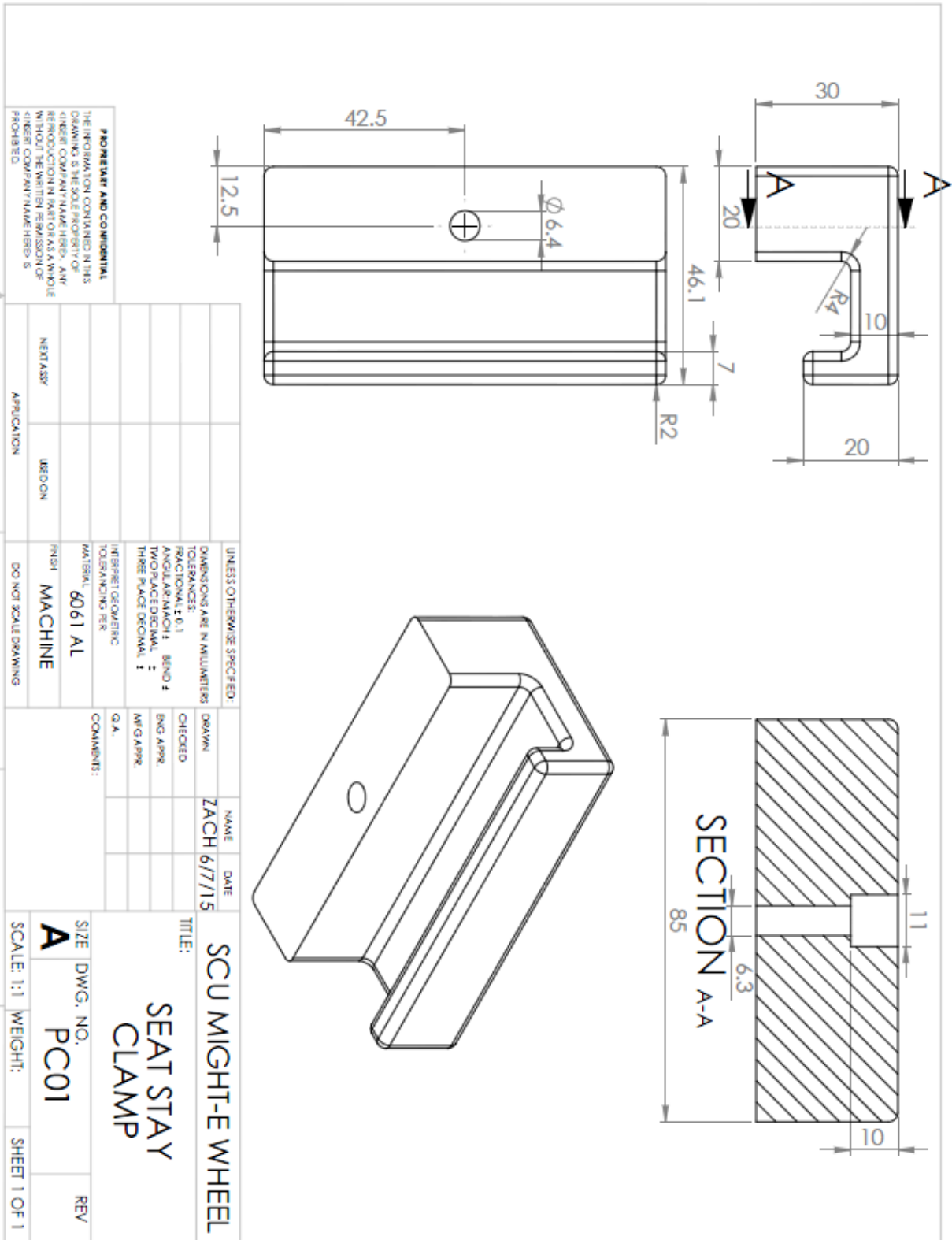
Figure J-6: Seat Stay Clamp Drawing
