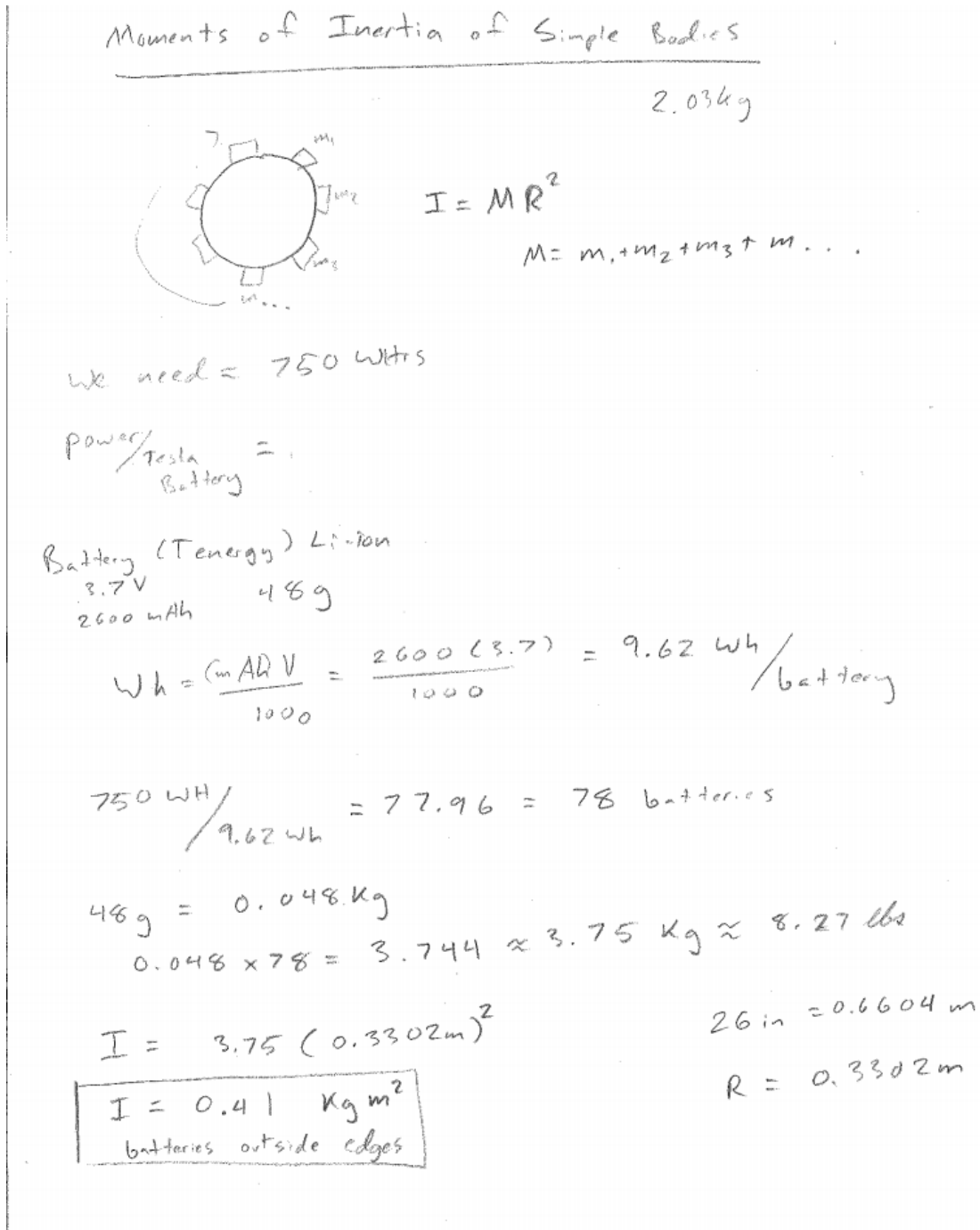
Figure E-1: Inertia Calculations
