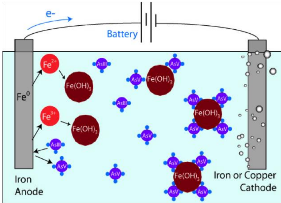
Figure 4: Electrocoagulation Process. (Source: University of California Berkeley, Gadgil Lab)
