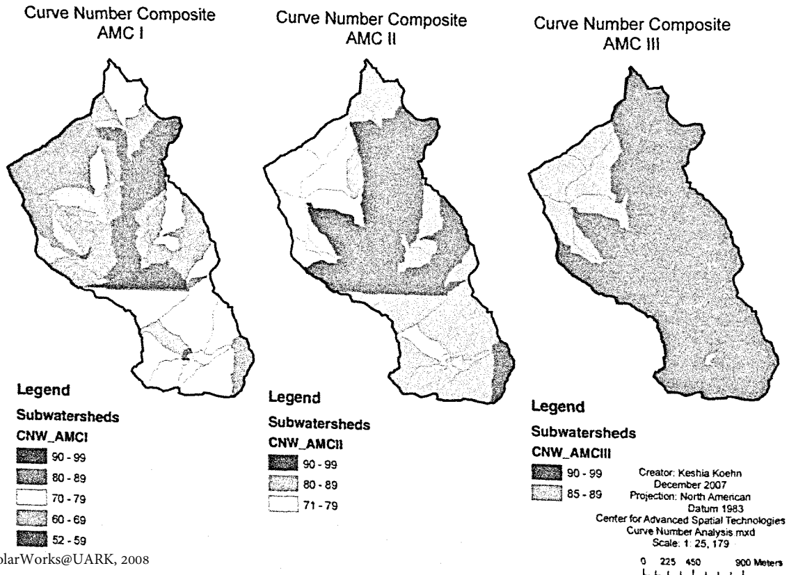
Figure 2. Sub-watershed weighted curve numbers for varied AMC levels. For each map, left to right, the AMC was increased, increasing the average sub-watershed CN and runoff depths.
