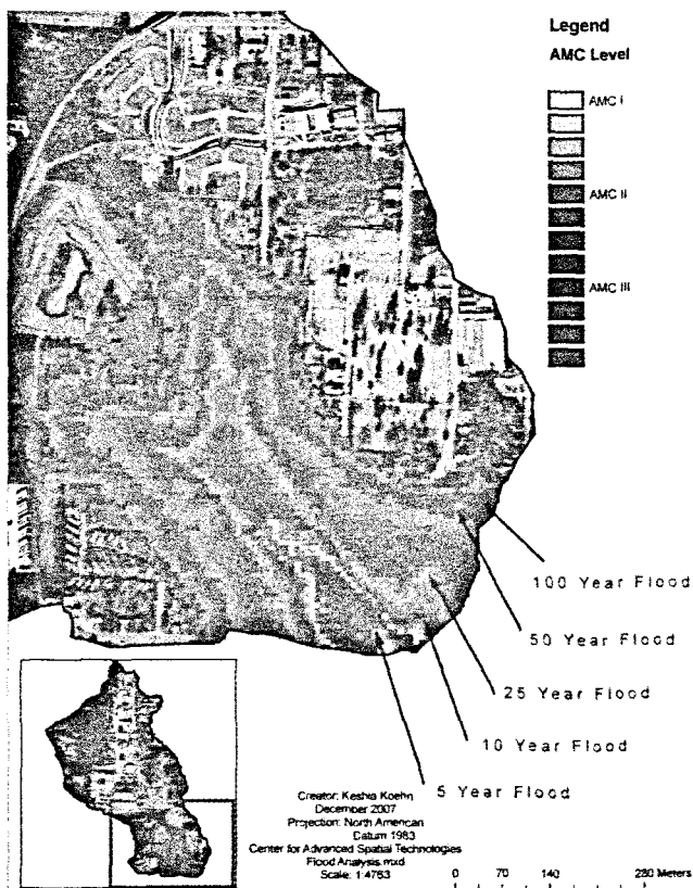
Figure 3. Maximum flooding extent for varied AMC levels showing the locations of potential flooding on aerial photography of the southern quadrant of the study area.
