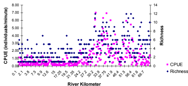
Figure 2. CPUE (individuals / min) and species richness of the qualitative survey of the Tyronza River, Arkansas, plotted by river kilometer. The survey began at river km 0, upstream, and ended at river km 70.4 at Parkin, Arkansas.
