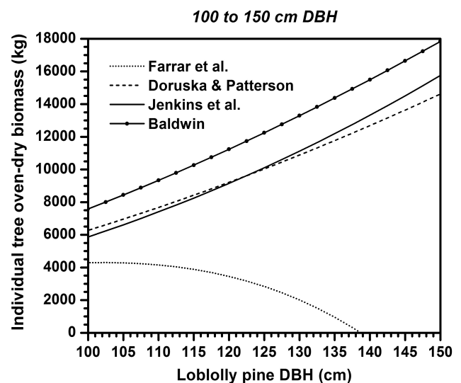
Figure 3. Predicted aboveground live-tree, oven-dry biomass as a function of stem diameter for loblolly pines between 100 and 150 cm DBH using the four different model systems. Note the dramatic departure of the Farrar et al. system from the others.
