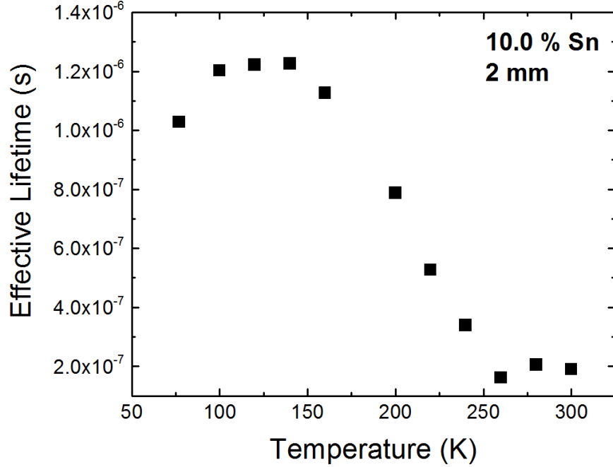
Figure 54: Effective lifetime of the 10.0% photoconductor with 1.6 mm electrode spacing (2 mm square mesa) calculated for each measured temperature.
