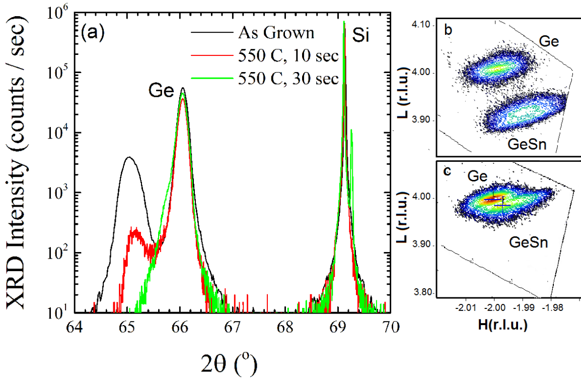
Figure 7: (a) The XRD rocking curves for \text{Ge}_{0.93}\text{Sn}_{0.07} represent the lattice constant change for 30 seconds at 550 °C and for 10 seconds at 550 °C compared to the as grown sample. Reciprocal space maps of the (b) as grown and (c) sample annealed at 550 °C for 30 seconds show \text{Ge}_{1-x}\text{Sn}_x film transition from partially relaxed to a reduced Sn mole fraction and relaxed film. Reproduced by permission of The Electrochemical Society [31].
