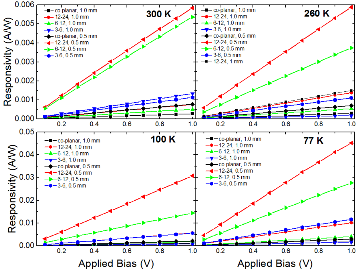
Figure 68: Responsivity measured for the Ge 0.93 Sn 0.07 interdigitated photoconductor devices at 1.55 \mu\text{m} for device temperatures of 300, 260, 100, and 77 K.
