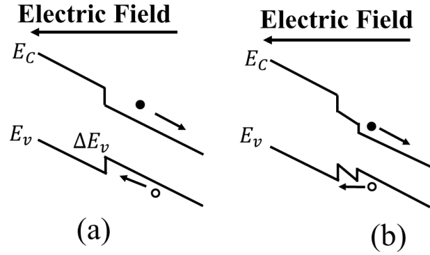
Figure 32: (a) Large band offset in the valence band ( \Delta E_v ) scatters high energy holes, but does not affect the electron. (b) Graded heterostructure reduces the overall energy step for the hole.
