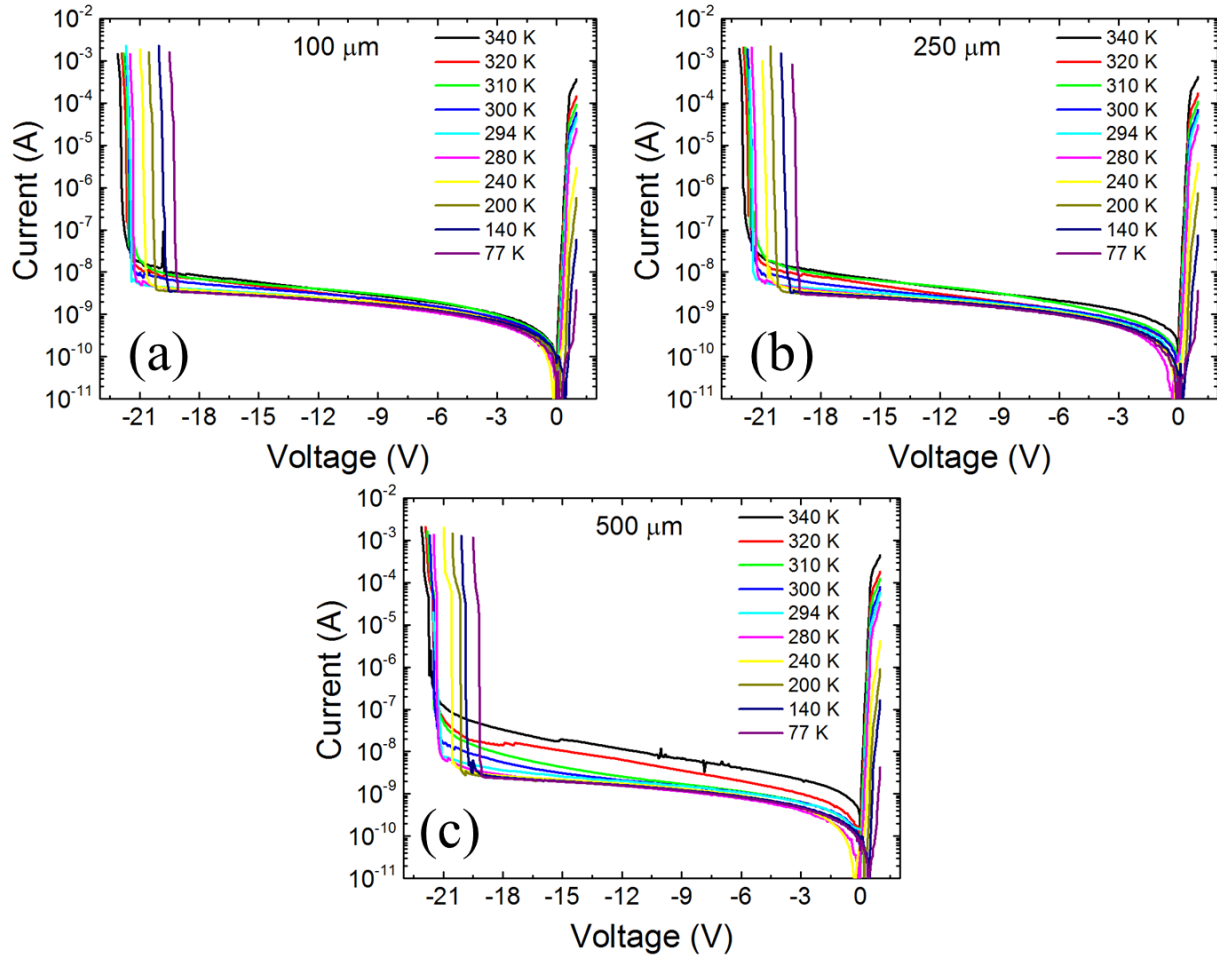
Figure 75: Dark I-V measurement of the (a) 100 \mu\text{m} , (b) 250 \mu\text{m} , and (c) 500 \mu\text{m} diameter \text{Ge}_{1-x}\text{Sn}_x APDs measured for temperatures from 340 to 77 K.
