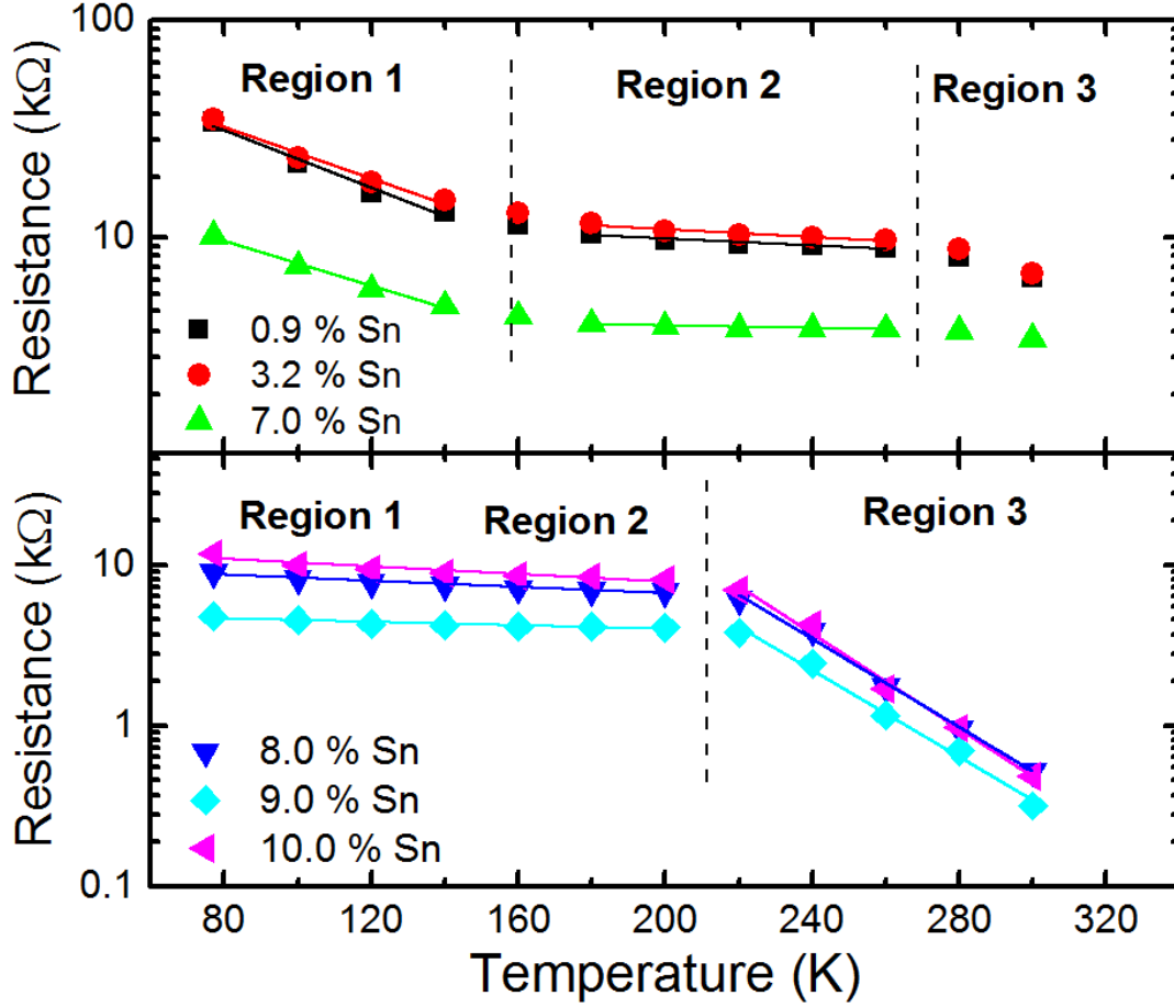
Figure 41: Dark resistance of each 2 mm \text{Ge}_{1-x}\text{Sn}_x photoconductor measured for varying temperature. Regions 1, 2, and 3 defined the regions of changing slope for each detector set.
