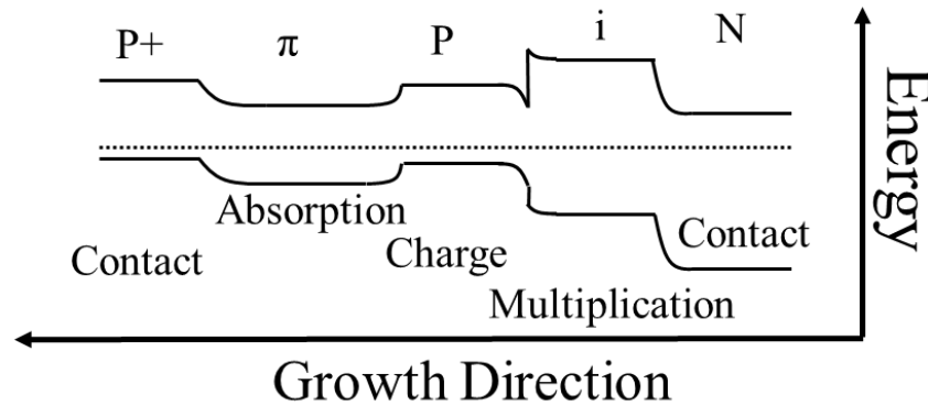
Figure 31: Band diagram for a SACM avalanche photodiode schematically shows the band offset and band bending for semiconductors with a type-I band alignment.
