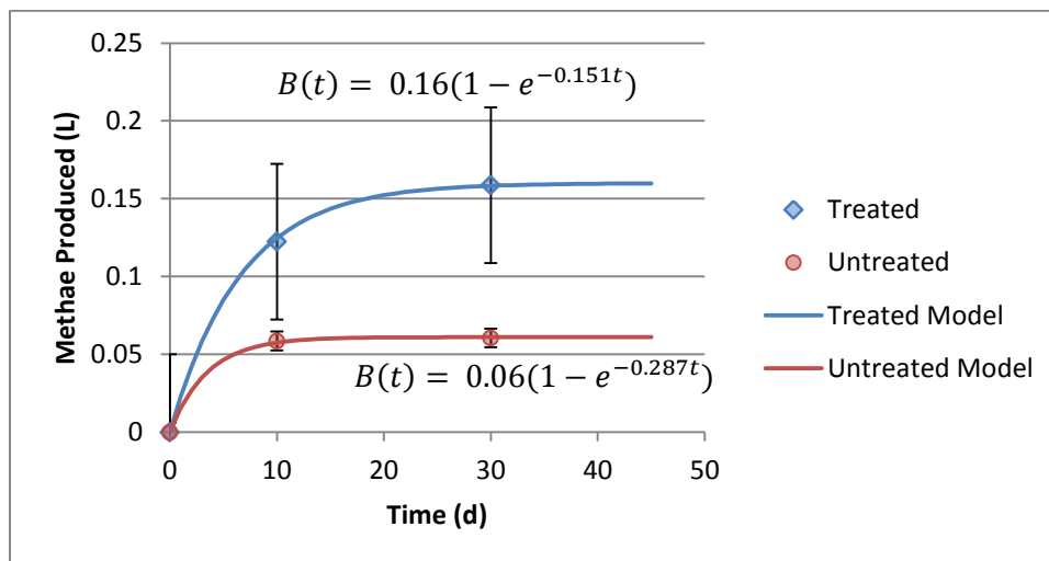
Figure 1: Graph used to determine the first-order kinetic rate constant for each case
