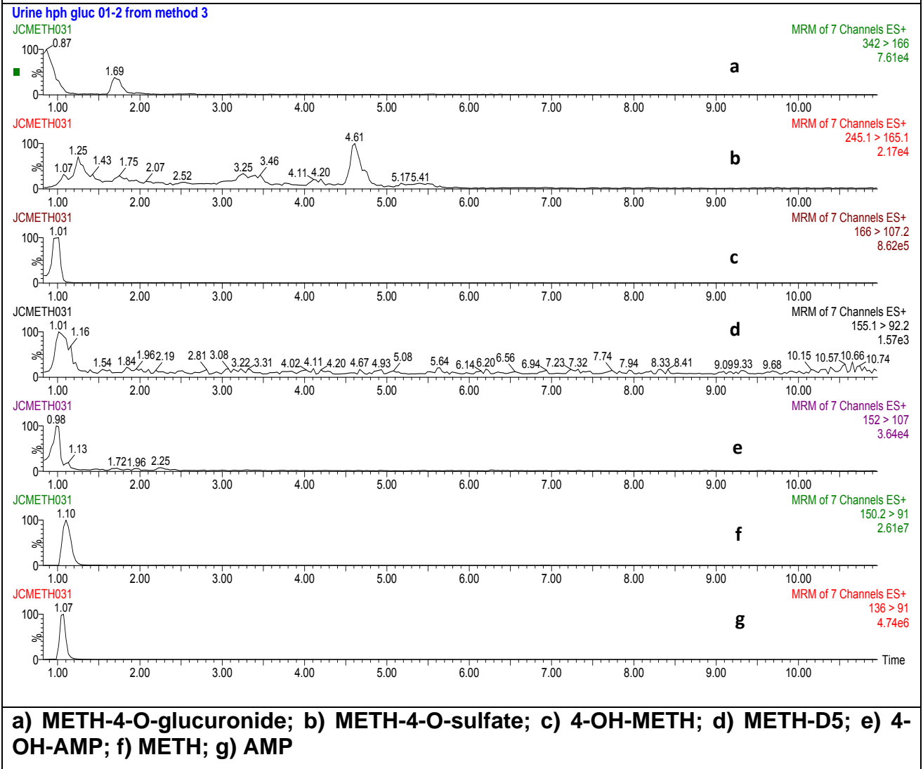
Figure 4: Method 3 Chromatogram
