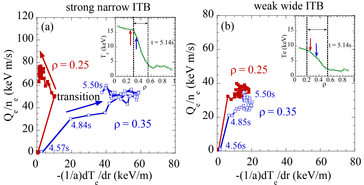
FIG.3. Heat flux normalized by electron density as a function of electron temperature gradient at electron internal transport barrier (ITB) region ( \rho = 0.35 ) and the boundary of ITB region ( \rho = 0.25 ) in the plasma with ECH (3MW in (a)) in negative magnetic shear configuration. There is no ITB formation when the ECH power is low (1.5MW in (b)) Radial profiles of electron temperature after the formation of ITB are also plotted. Dashed lines represent the ITB region while the arrows indicate the location where the dynamic transport analysis is applied for t = 4.57 - 5.5 sec .
