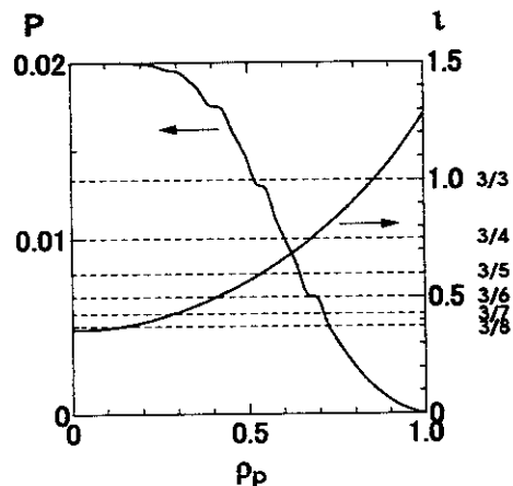
FIG.4. A marginally stable pressure profile against the n = 3 pressure driven mode with the flat pressure regions given by w = 0.03 at \iota = 3/7, w = 0.03 at \iota = 3/6, w = 0.02 at \iota = 3/5 and w = 0.02 at \iota = 3/4 . The rotational transform profile obtained by VMEC code, and rational surfaces with \iota = 3/3, 3/4, 3/5, 3/6, 3/7, 3/8 are shown.
