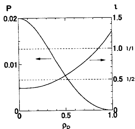
FIG.1. An assumed pressure profile and a rotational transform profile in the LHD configuration with the inward magnetic axis shift of 25cm obtained by VMEC code[18]. Dotted lines show \iota = 1/1 and \iota = 1/2 , respectively. The central beta value is \beta(0) = 2\% and the average beta value is \bar{\beta} = 0.632\% . The radius \rho_p denotes a square root of normalized poloidal flux, which is also used in FIG.2 - FIG.4.
