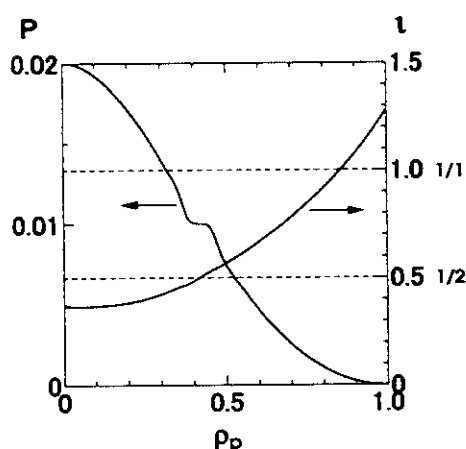
FIG.2. A marginally stable pressure profile against the n = 1 pressure driven mode with the width of flat pressure region w = 0.045 . The rotational transform profile obtained by VMEC code, and rational surfaces with \iota = 1/1 and \iota = 1/2 are also shown.
