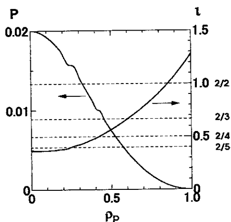
FIG.3. A marginally stable pressure profile against the n = 2 pressure driven mode with the flat pressure regions given by w = 0.04 at \iota = 2/5 and w = 0.02 at \iota = 2/4 . The rotational transform profile obtained by VMEC code, and rational surfaces with \iota = 2/2, 2/3, 2/4, 2/5 are shown.
