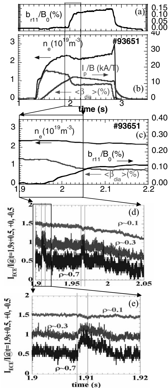
Fig. 1 The time evolution of the perturbed magnetic field (a,c), the electron density, the beta value and the net toroidal plasma current (b, c), and the electron temperature (d, e) in the discharge with the collapse.
