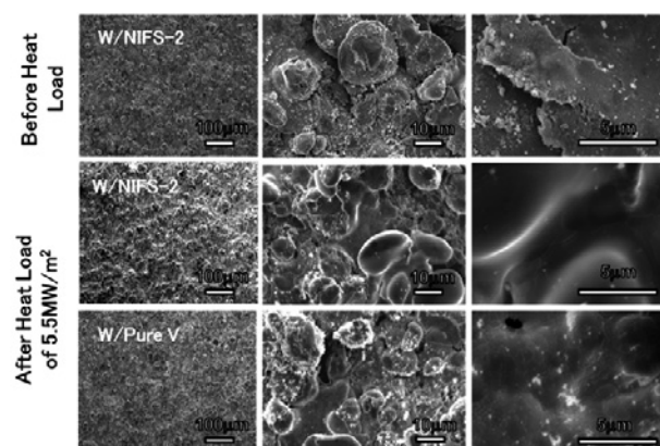
Fig.3. SEM images showing surface morphology of VPS-W on NIFS-HEAT-2. In the figure, VPS-W on pure V is also shown for comparison.
