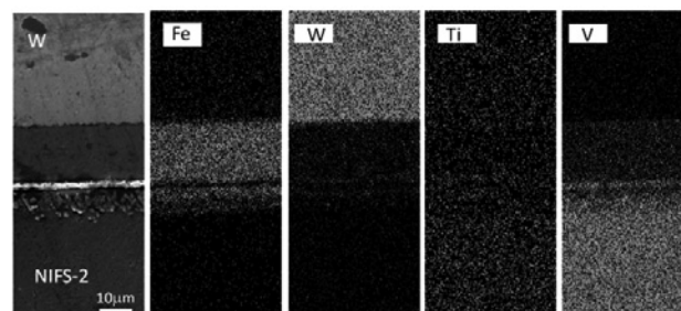
Fig.1. SEM images of interface between NIFS-HEAT-2 and brazed W.
