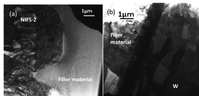
Fig.2. Microstructure of the interface between NIFS-HEAT-2 and brazed W (a) NIFS-HEAT-2 side (b) W-side
