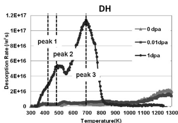
Fig. 3 DH desorption rate in recrystallized W(pre-irradiation 2.4MeV-Cu 2+ , irradiated at room temp. up to 1dpa)
