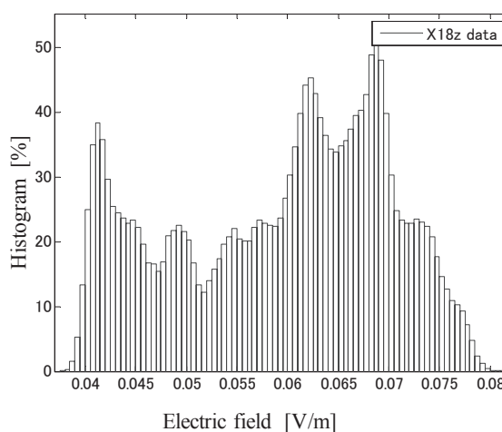
Fig. 2 PDF or histogram of leaked electric field within one burst period.
